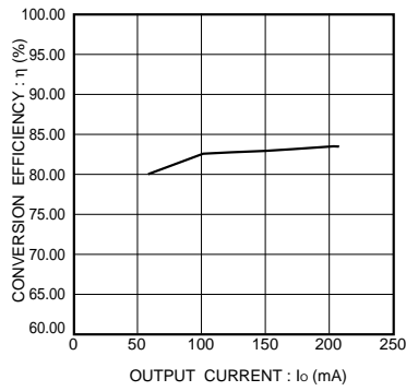
Fig.16 Conversion efficiency
