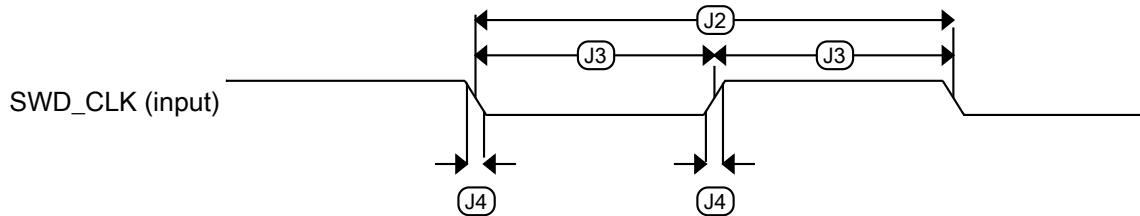
Figure 3. Serial wire clock input timing
