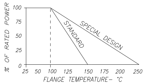
DERATING CURVE:
