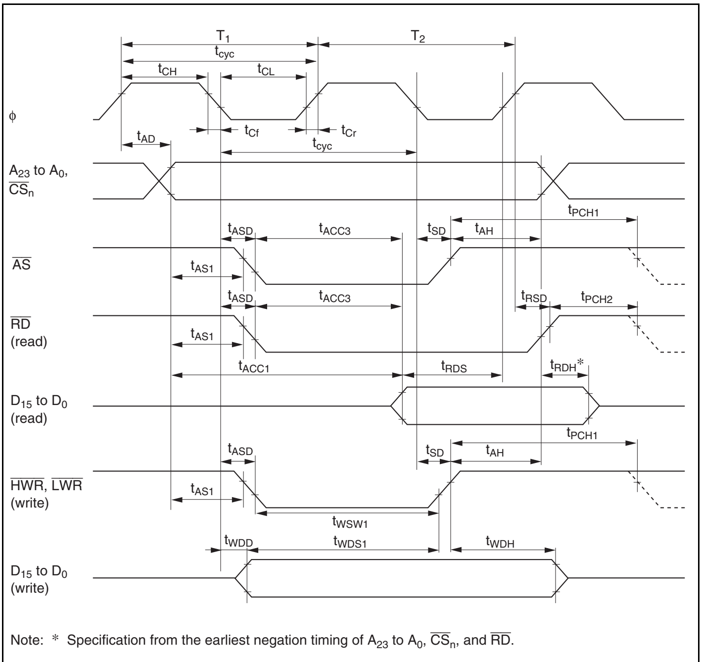
Figure 19.7 Basic Bus Cycle: Two-State Access
