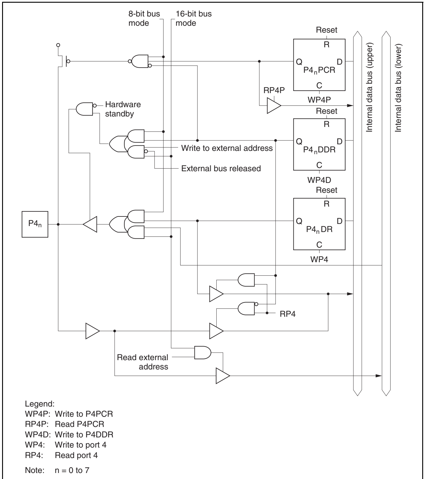
Figure C.1 Port 4 Block Diagram
