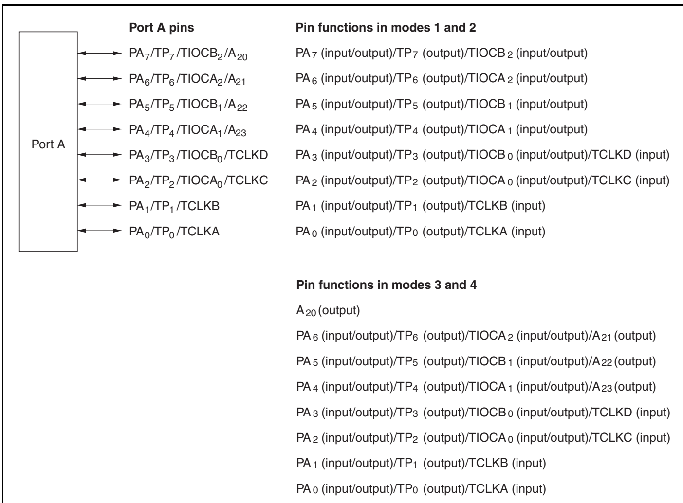
Figure 7.6 Port A Pin Configuration
