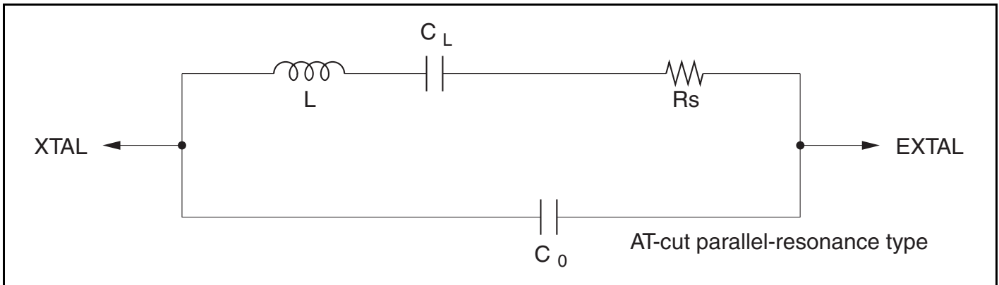
Figure 17.3 Crystal Resonator Equivalent Circuit
