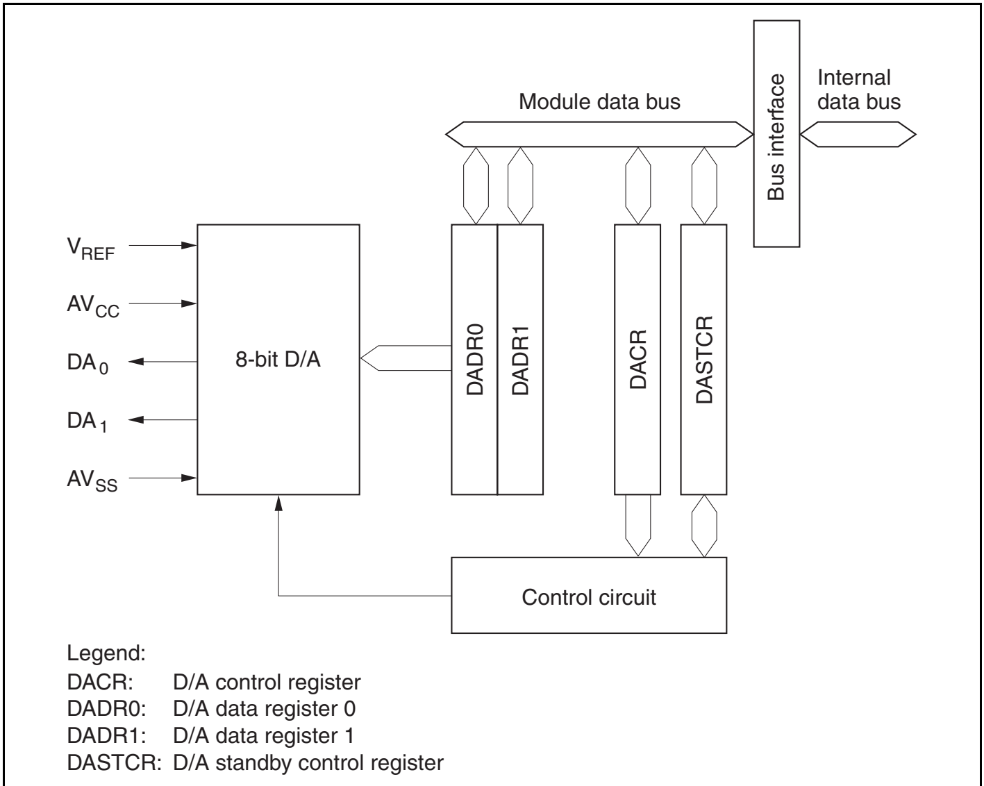
Figure 15.1 D/A Converter Block Diagram
