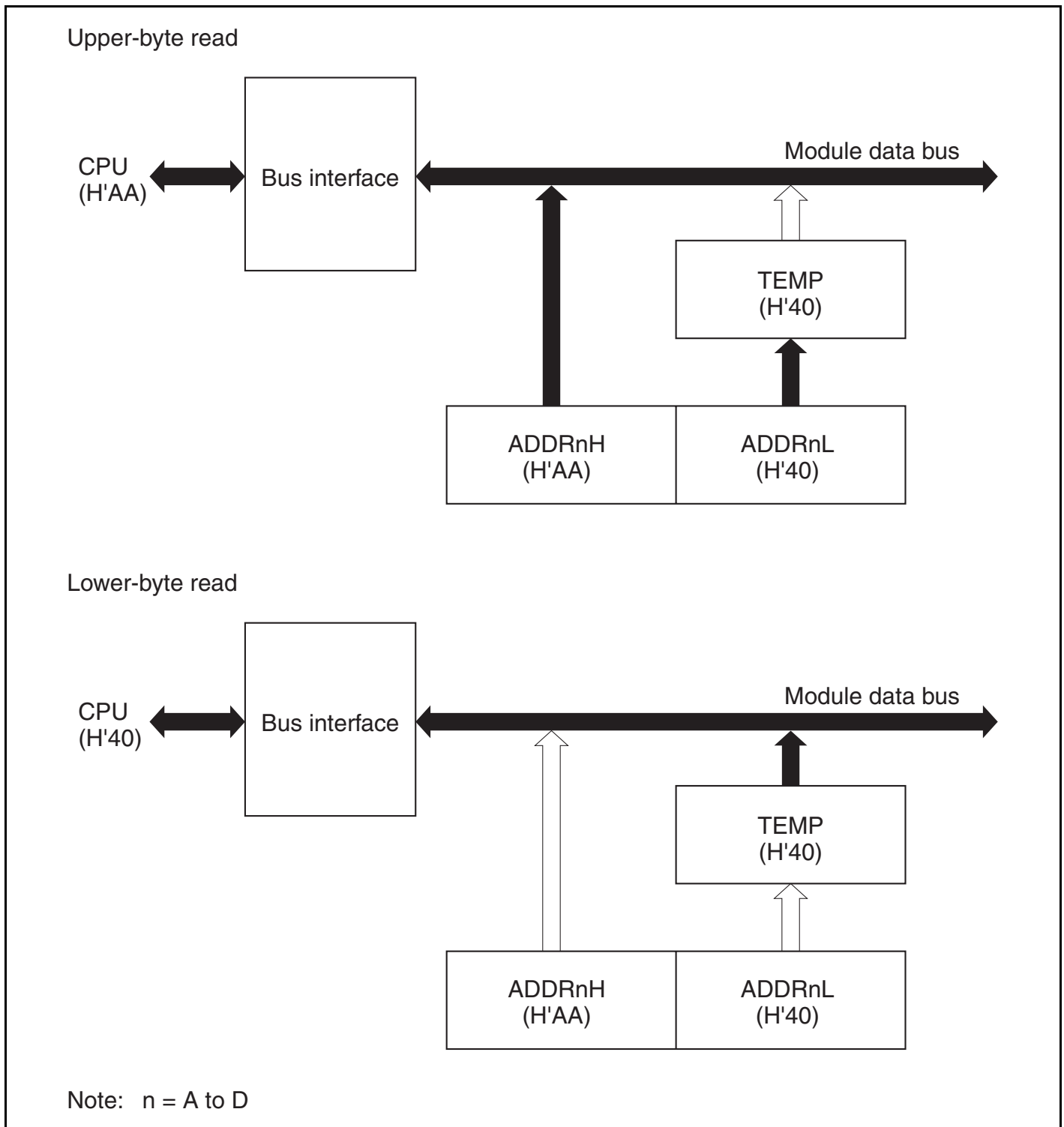
Figure 14.2 A/D Data Register Access Operation (Reading H'AA40)
