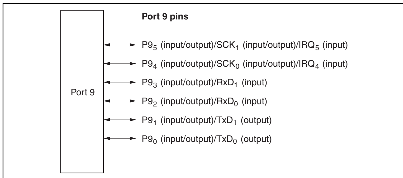
Figure 7.5 Port 9 Pin Configuration
