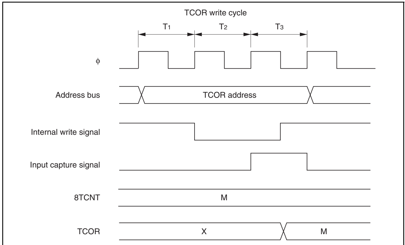
Figure 9.23 Contention between TCOR Write and Input Capture
