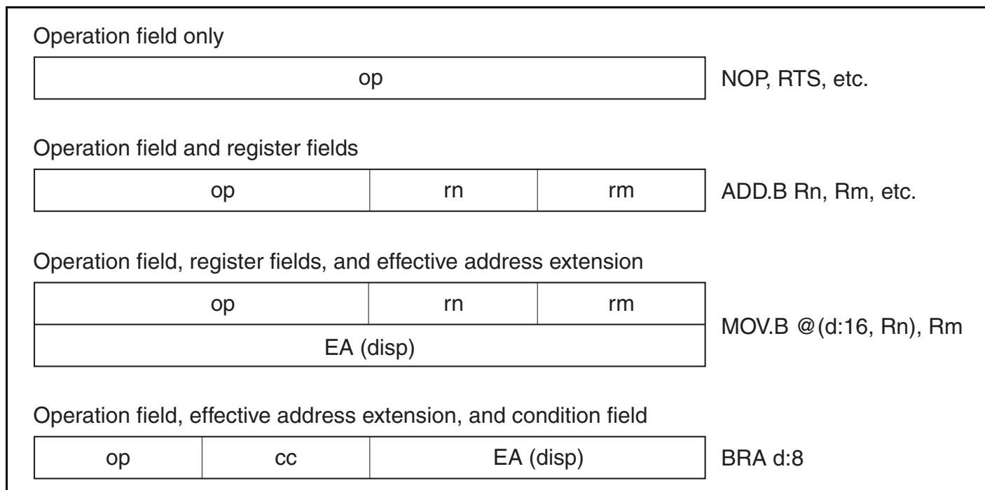
Figure 2.9 Instruction Formats
