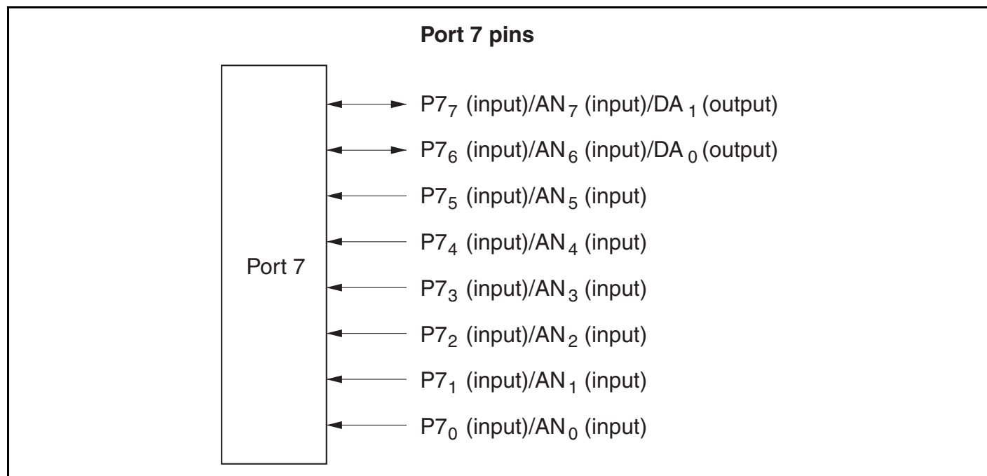
Figure 7.3 Port 7 Pin Configuration
