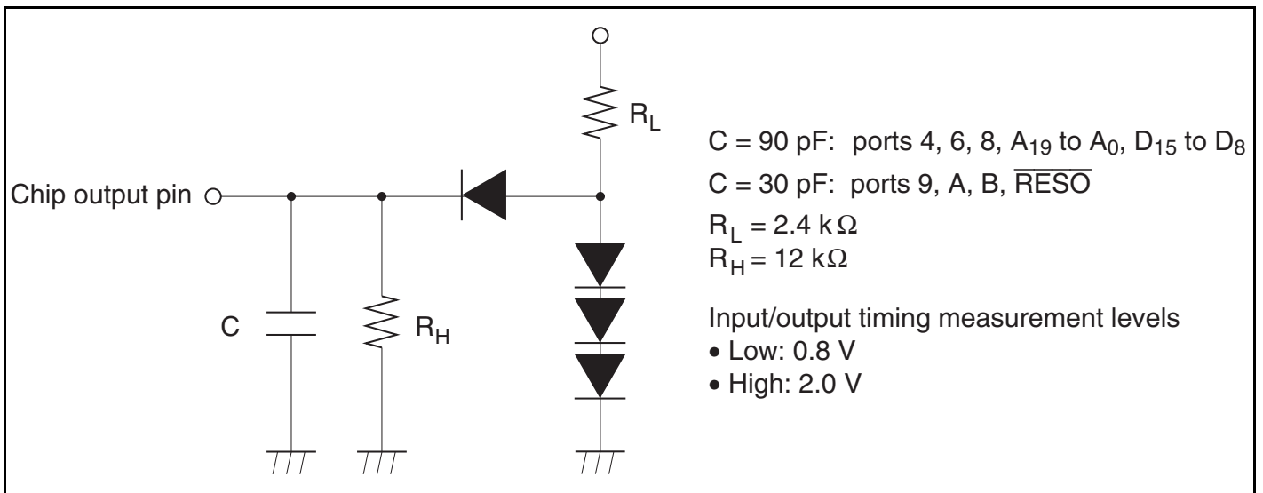
Figure 19.2 Output Load Circuit
