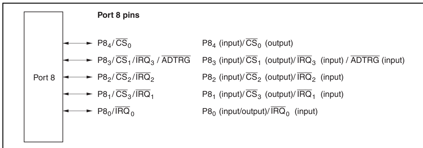
Figure 7.4 Port 8 Pin Configuration
