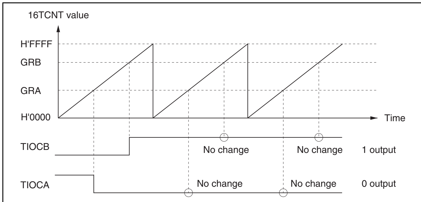
Figure 8.18 0 and 1 Output (TOA = 1, TOB = 0)
