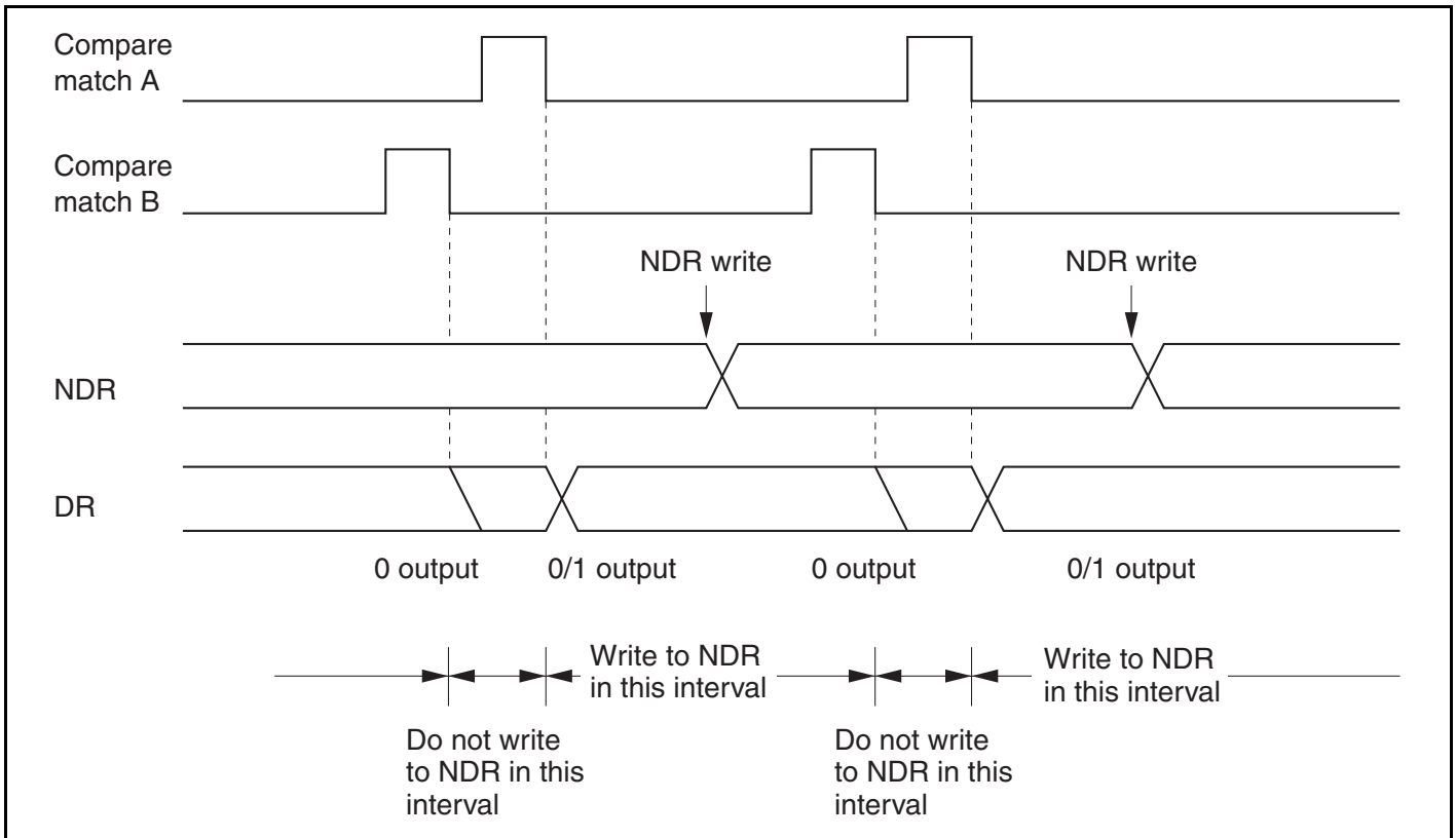
Figure 10.10 Non-Overlapping Operation and NDR Write Timing
