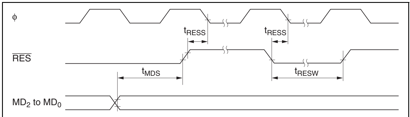
Figure 19.4 Reset Input Timing
