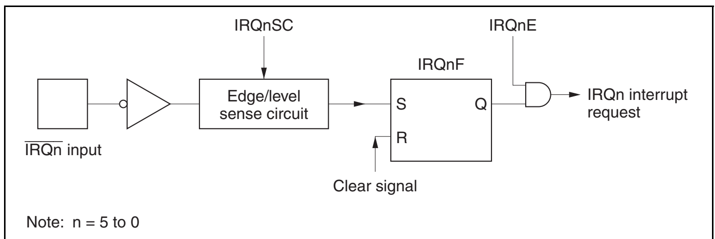
Figure 5.2 Block Diagram of Interrupts IRQ_5 to IRQ_0
