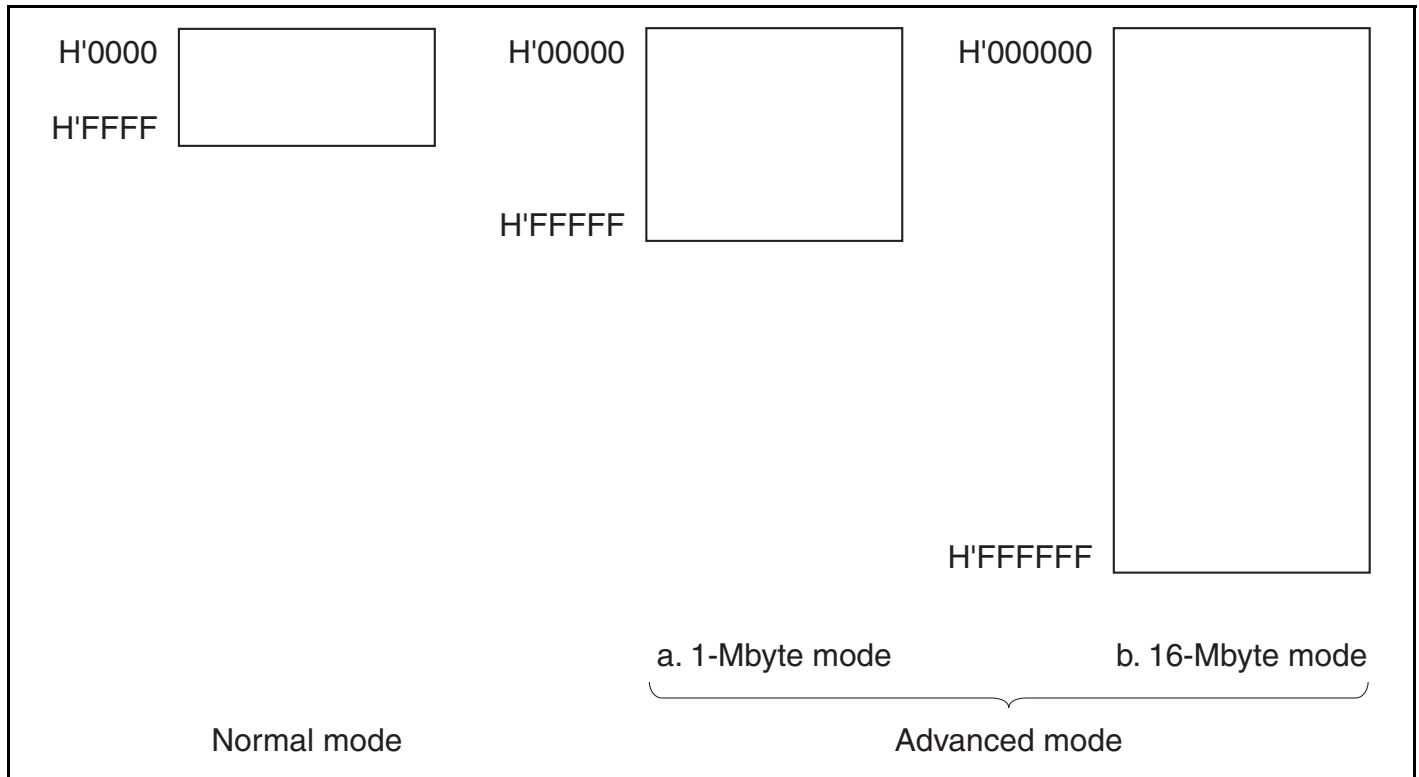
Figure 2.2 Memory Map
