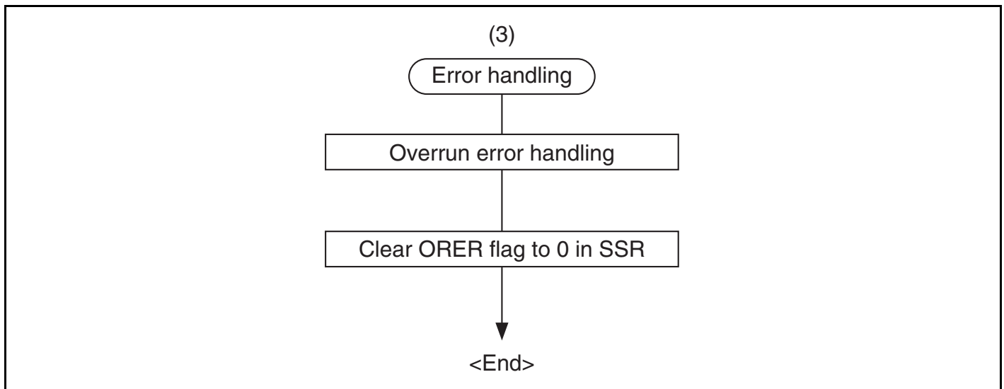
Figure 12.18 Sample Flowchart for Serial Receiving (2)
