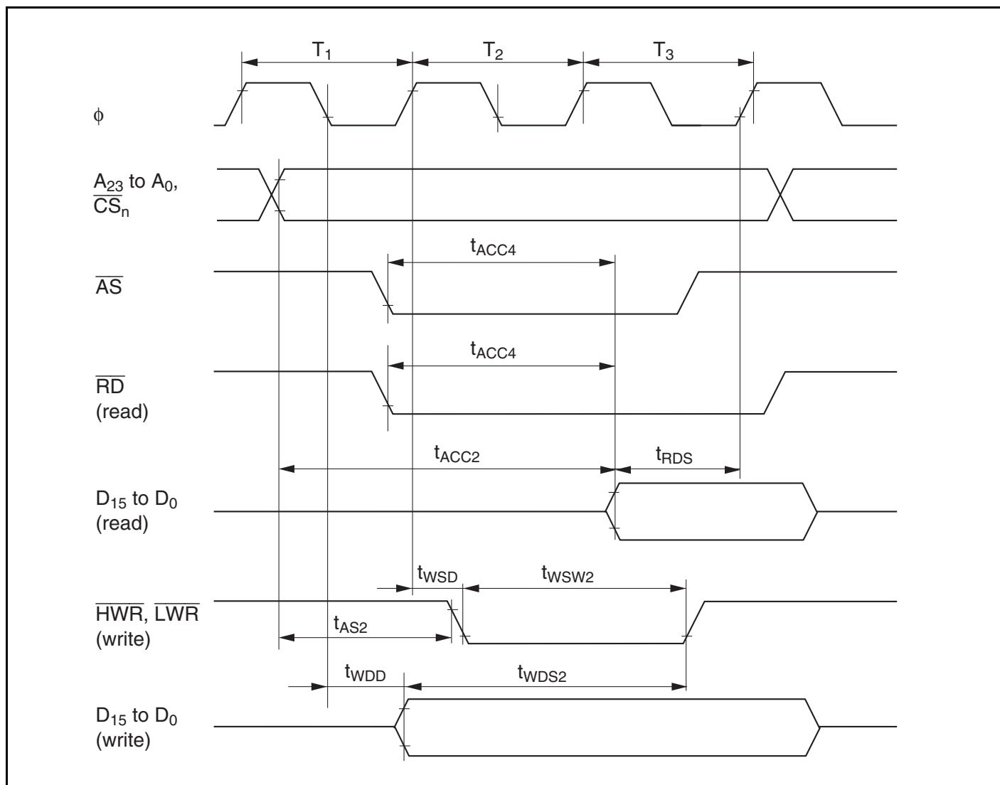
Figure 19.8 Basic Bus Cycle: Three-State Access
