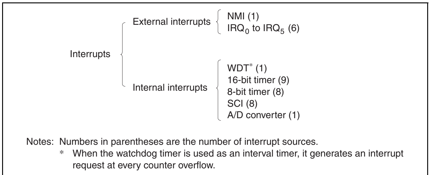
Figure 4.4 Interrupt Sources and Number of Interrupts
