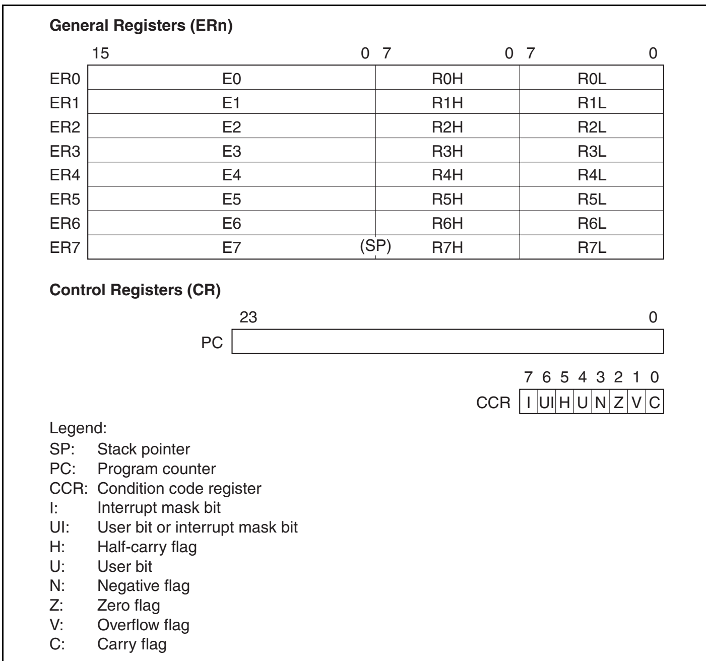
Figure 2.3 CPU Registers
