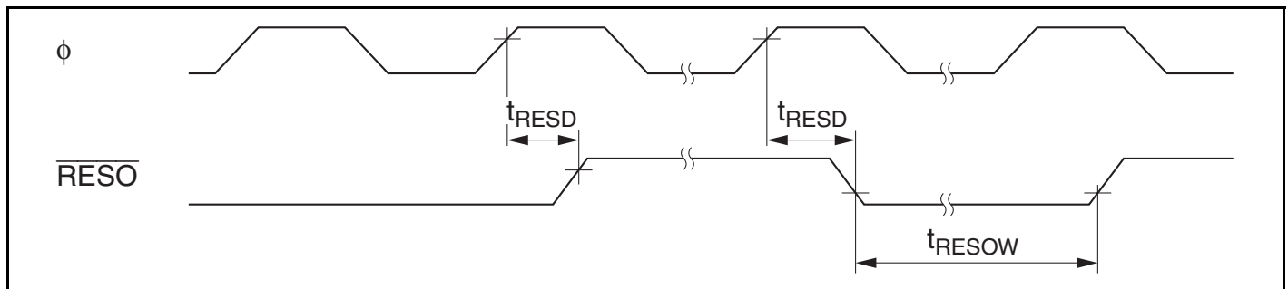
Figure 19.5 Reset Output Timing
