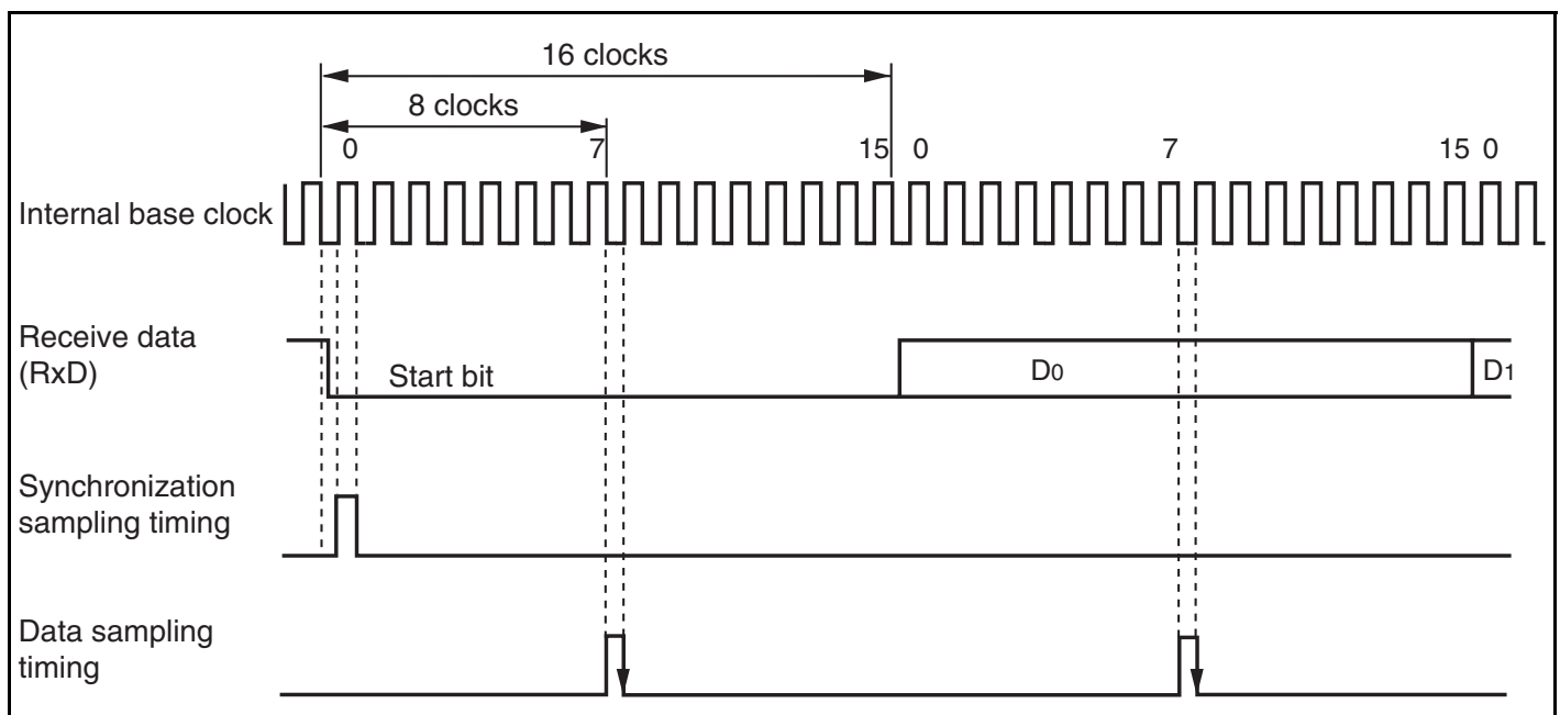
Figure 12.21 Receive Data Sampling Timing in Asynchronous Mode
