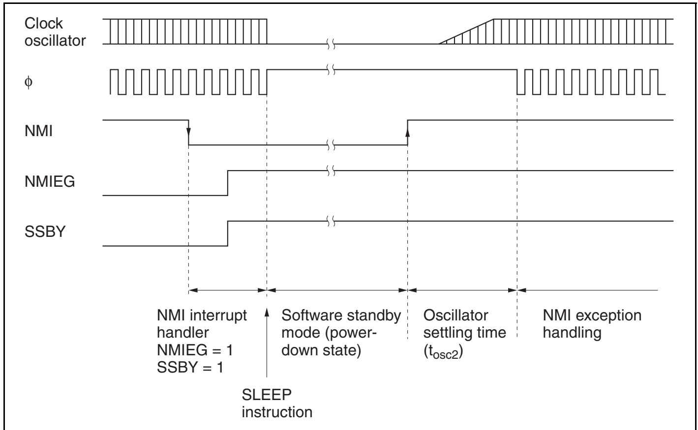
Figure 18.1 NMI Timing for Software Standby Mode (Example)
