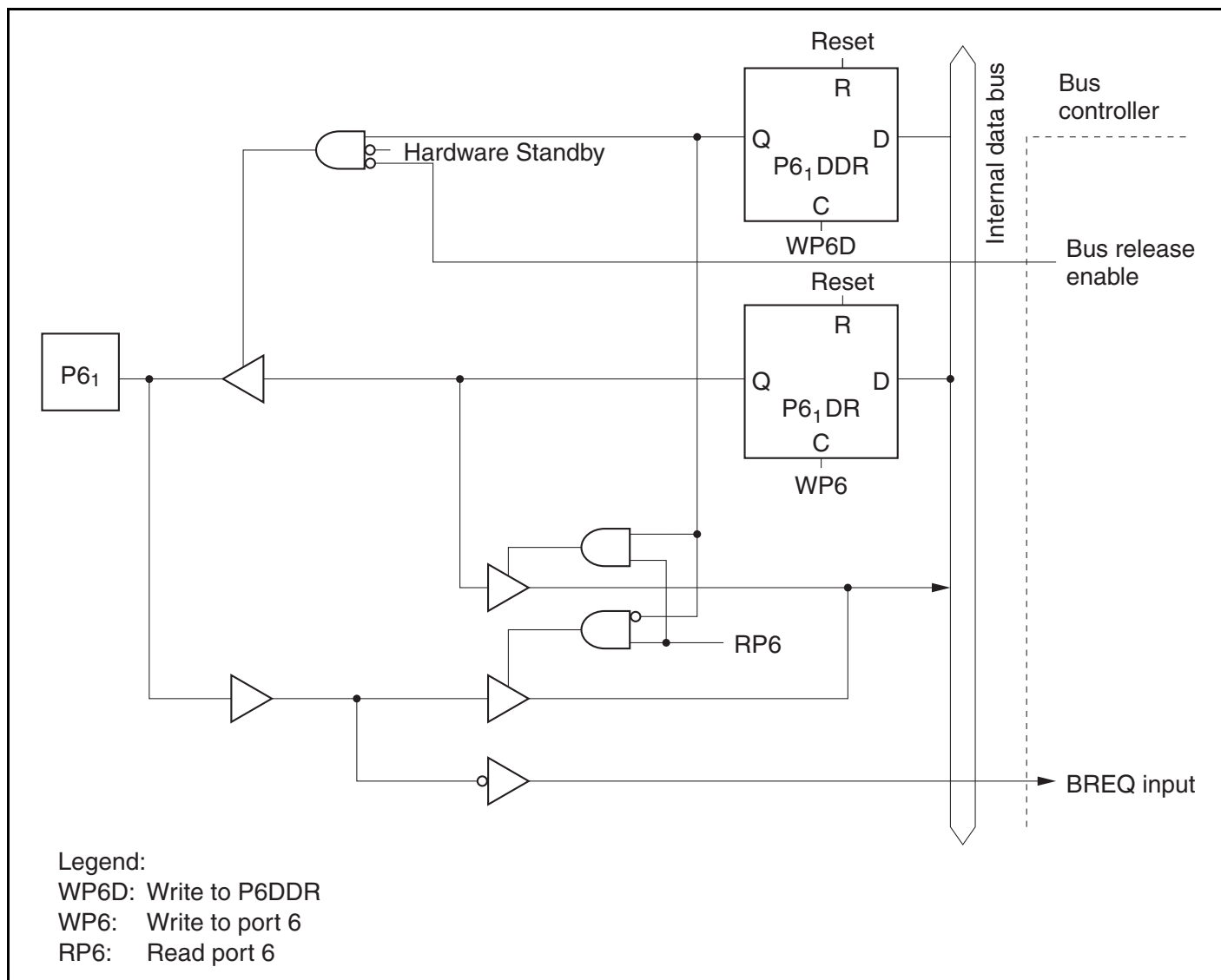
Figure C.2 (b) Port 6 Block Diagram (Pin P6 1 )
