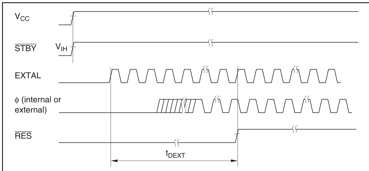
Figure 17.7 External Clock Output Settling Delay Timing
