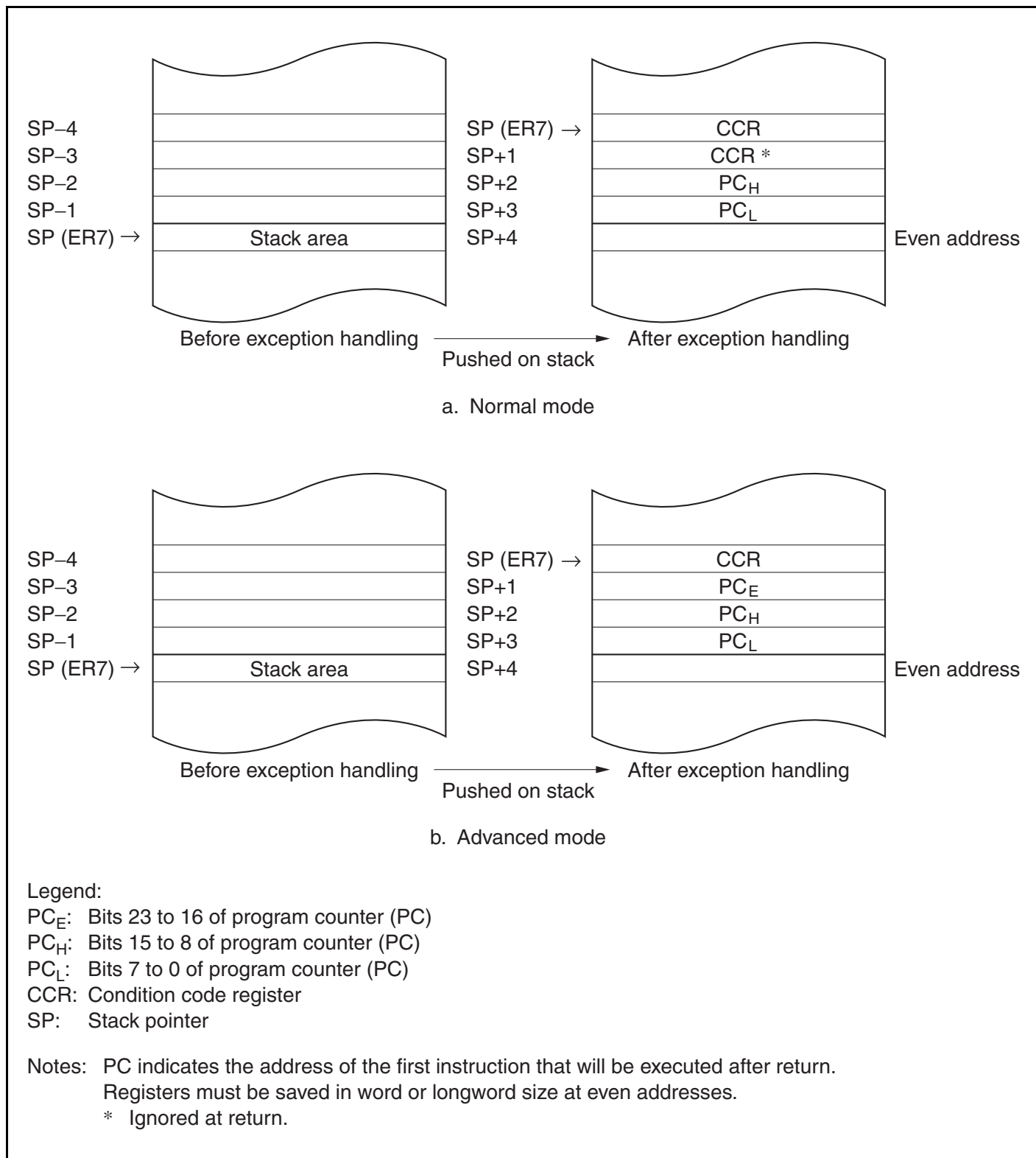
Figure 4.5 Stack after Completion of Exception Handling
