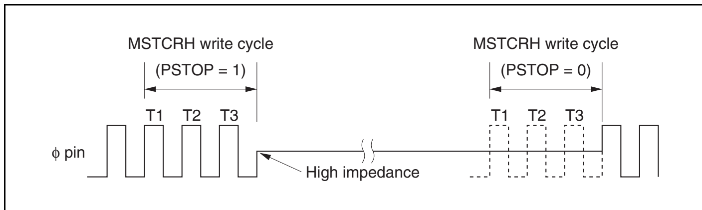
Figure 18.3 Starting and Stopping of System Clock Output
