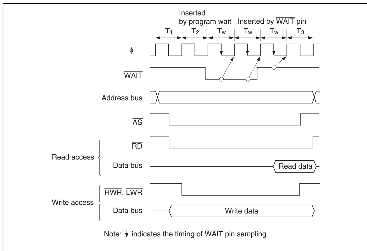
Figure 6.17 Example of Wait State Insertion Timing
