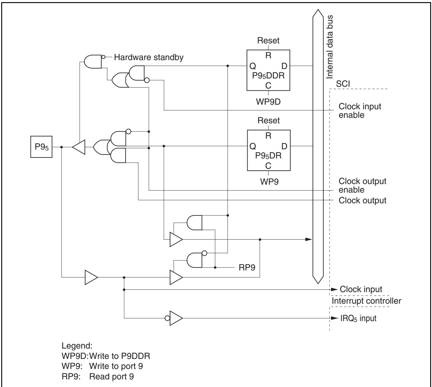
Figure C.5 (f) Port 9 Block Diagram (Pin P9 5 )
