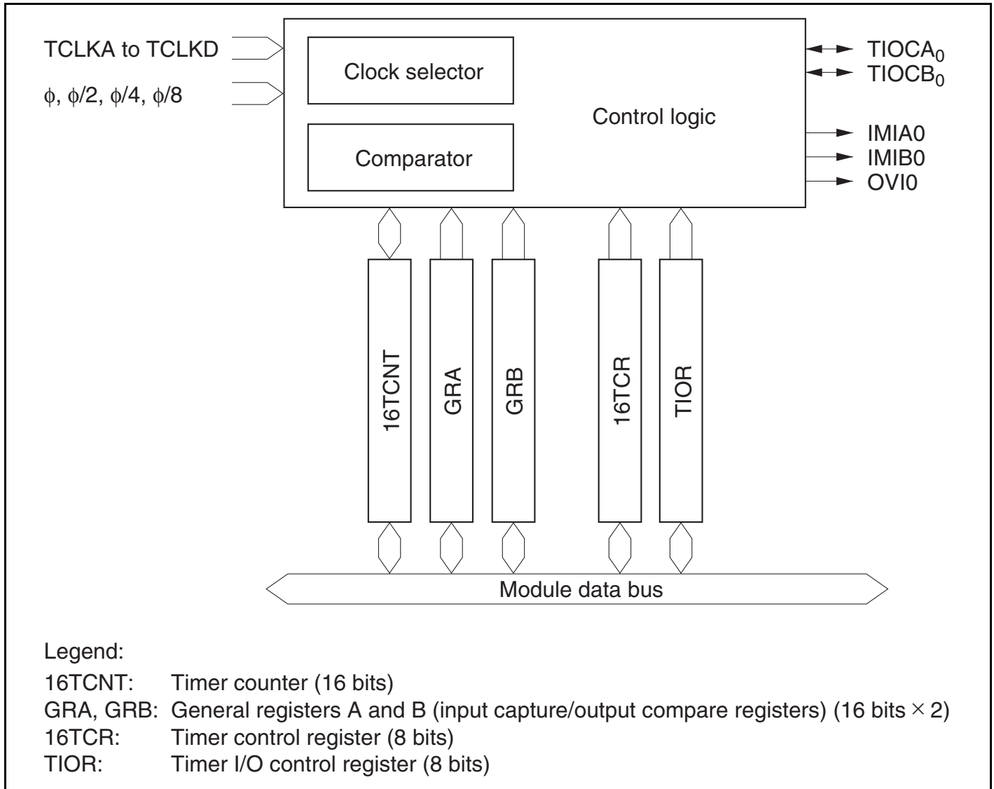
Figure 8.2 Block Diagram of Channels 0 and 1
