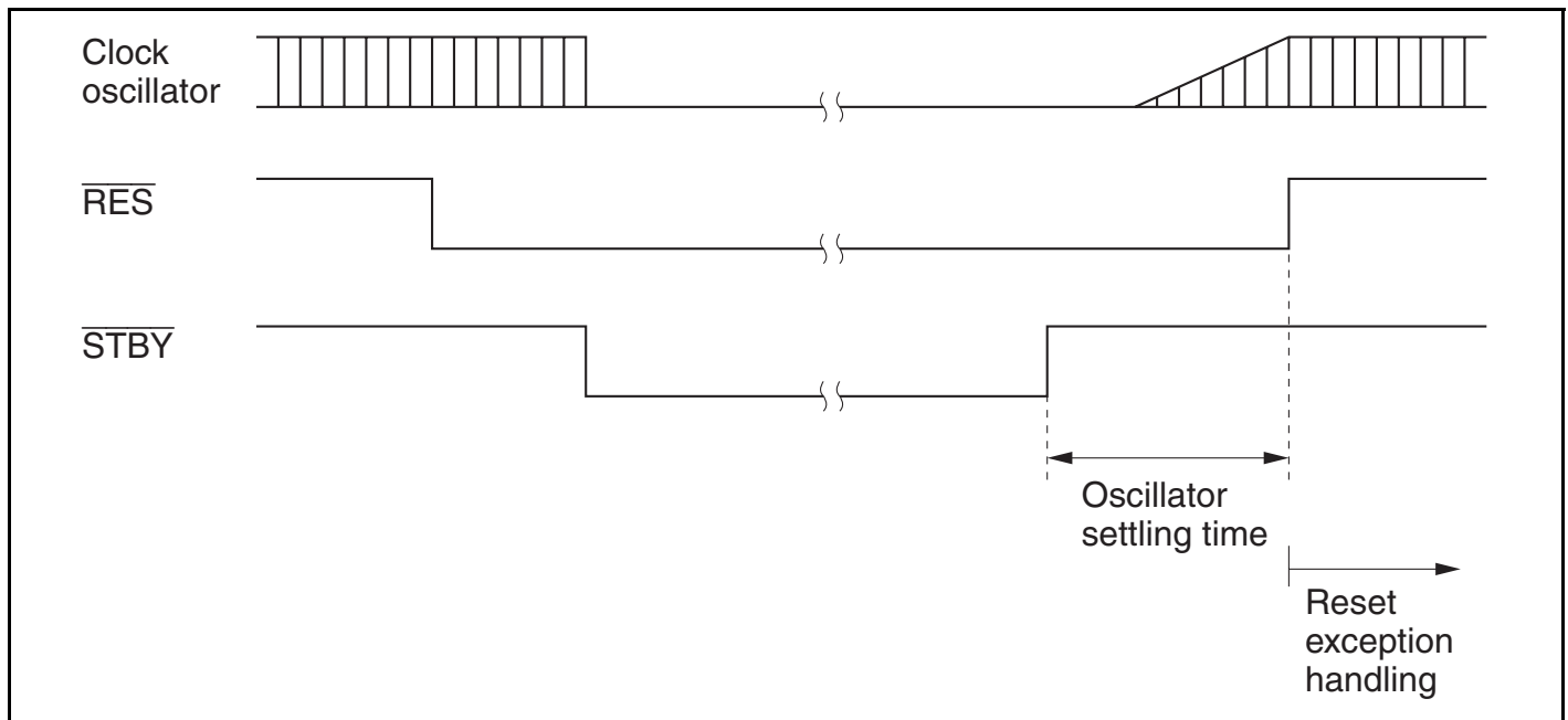
Figure 18.2 Hardware Standby Mode Timing
