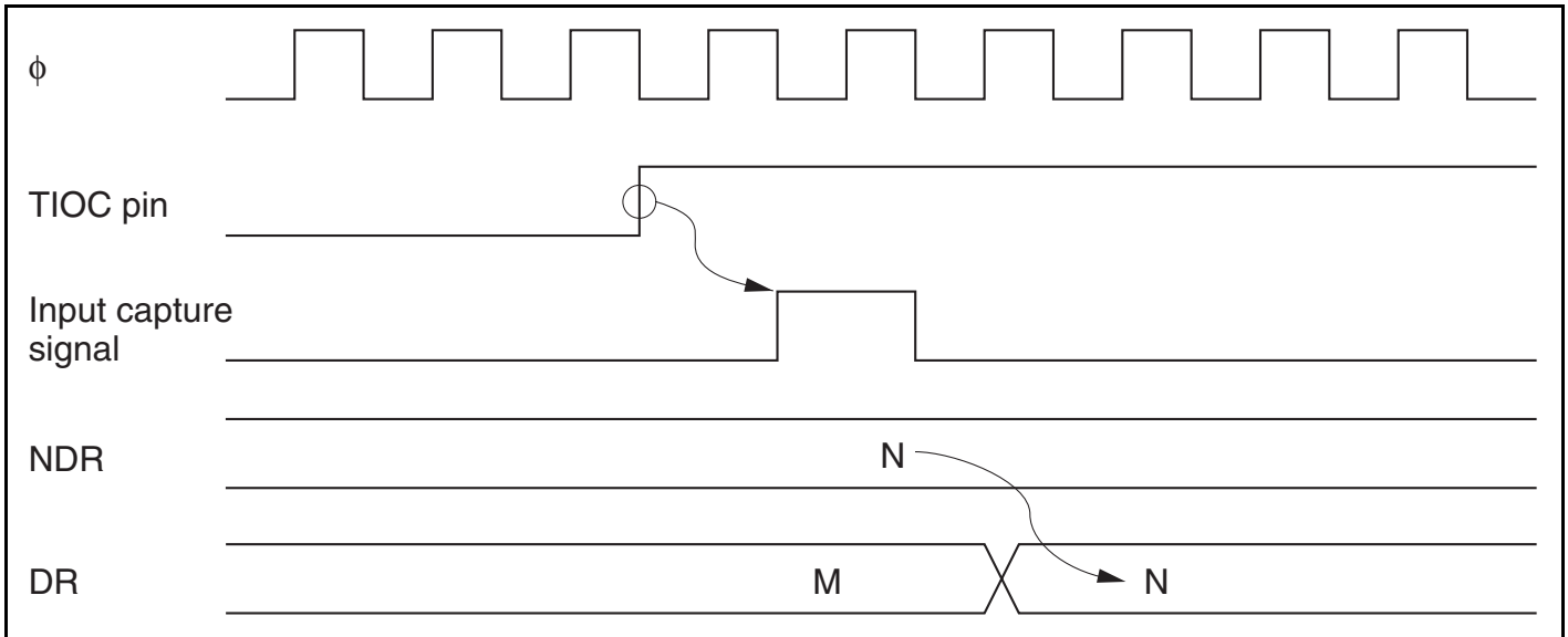
Figure 10.8 TPC Output Triggering by Input Capture (Example)
