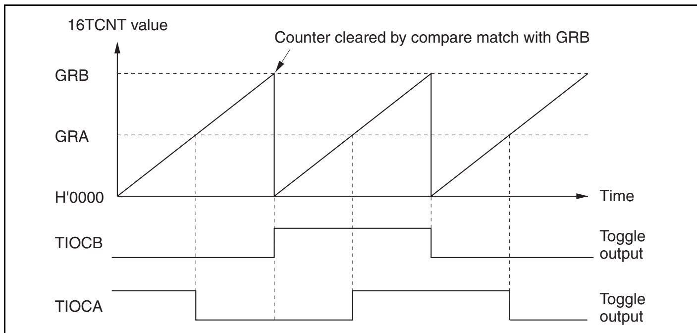
Figure 8.19 Toggle Output (TOA = 1, TOB = 0)
