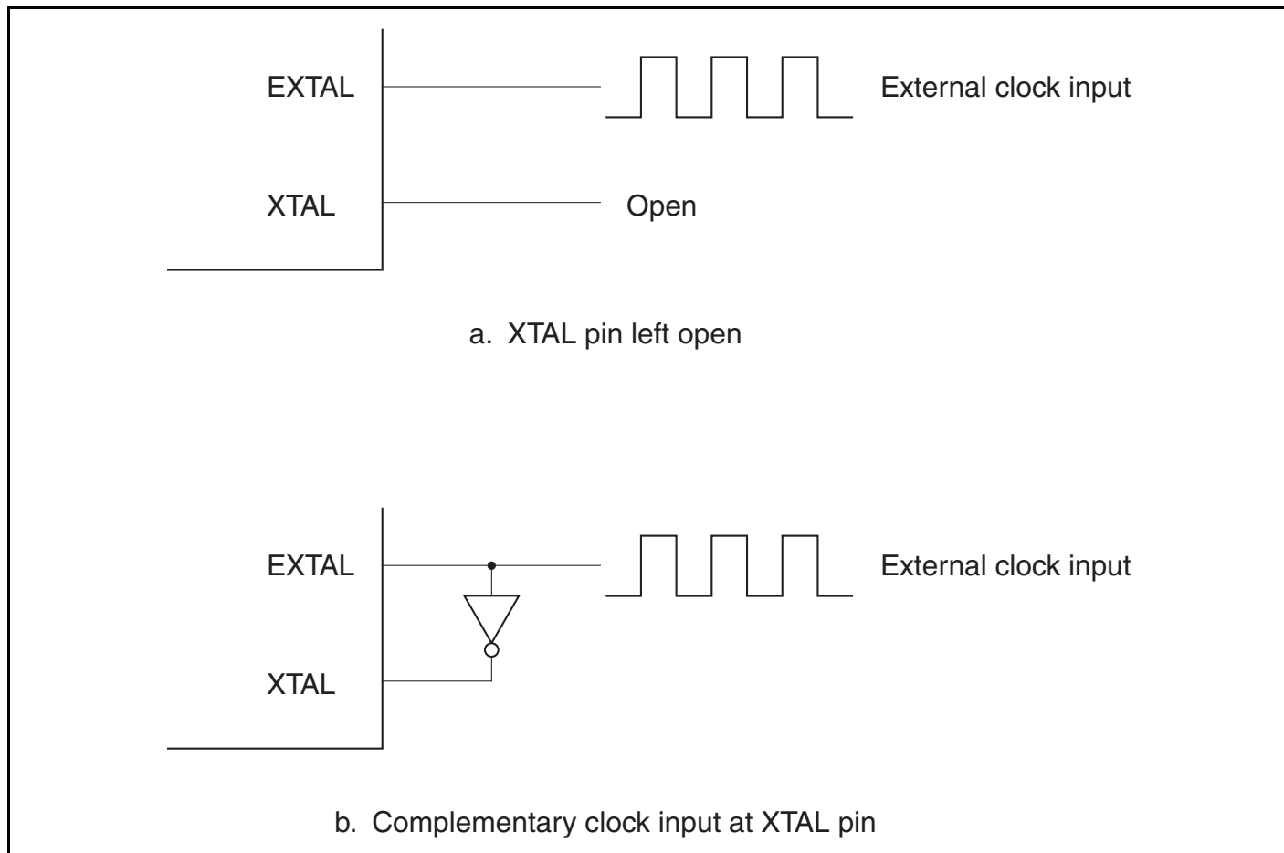
Figure 17.5 External Clock Input (Examples)
