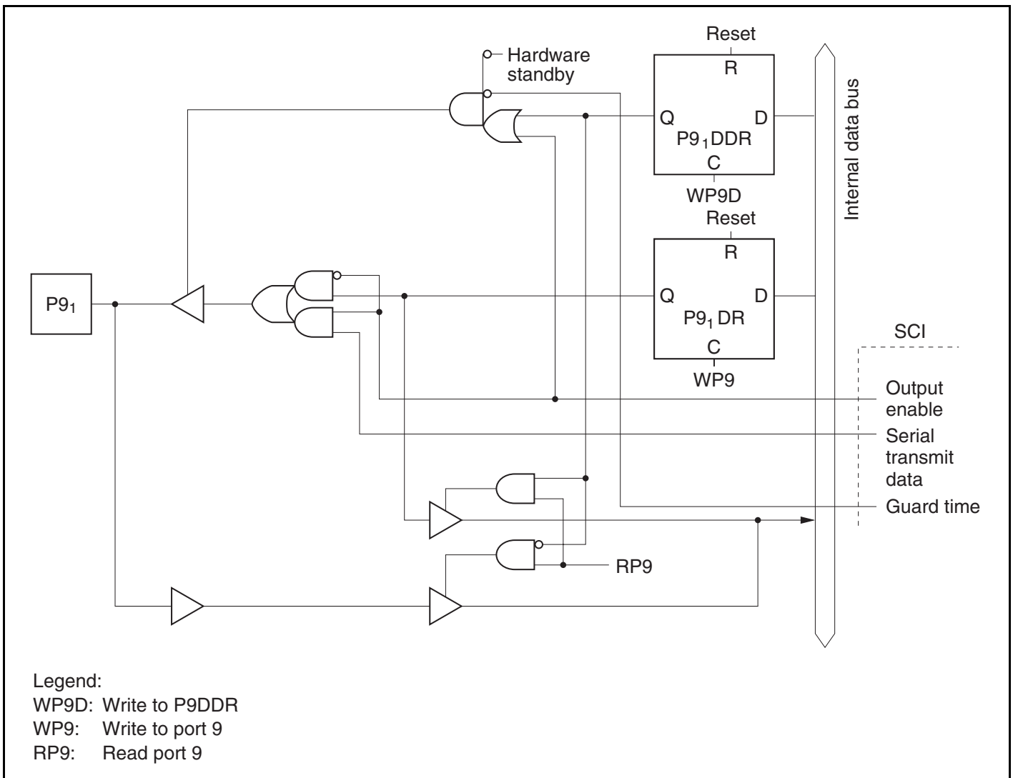
Figure C.5 (b) Port 9 Block Diagram (Pin P9 1 )
