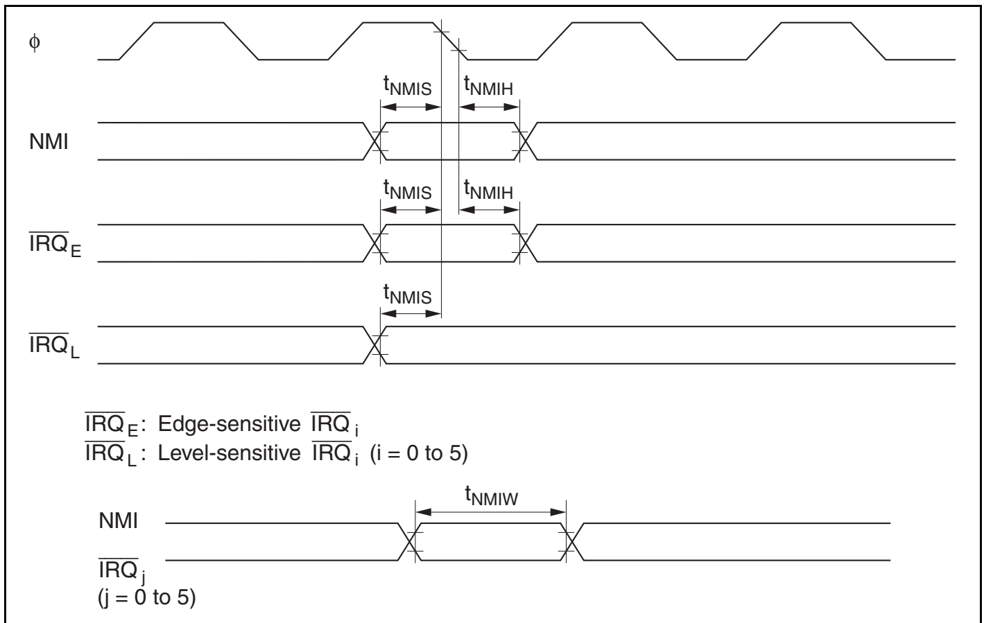
Figure 19.6 Interrupt Input Timing
