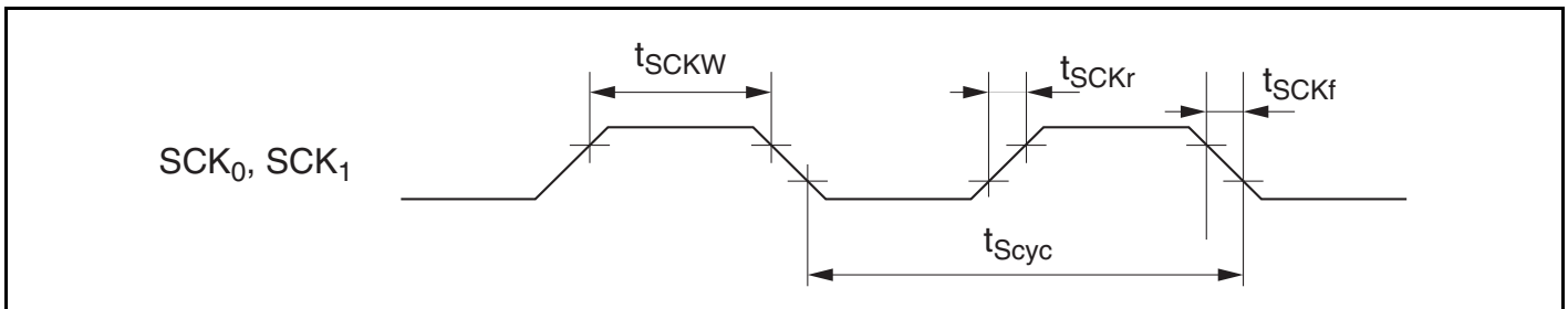
Figure 19.14 SCI Input Clock Timing
