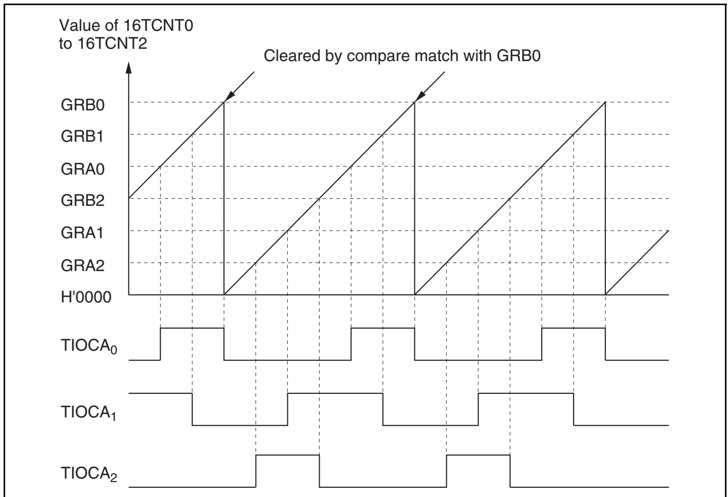
Figure 8.25 Synchronization (Example)
