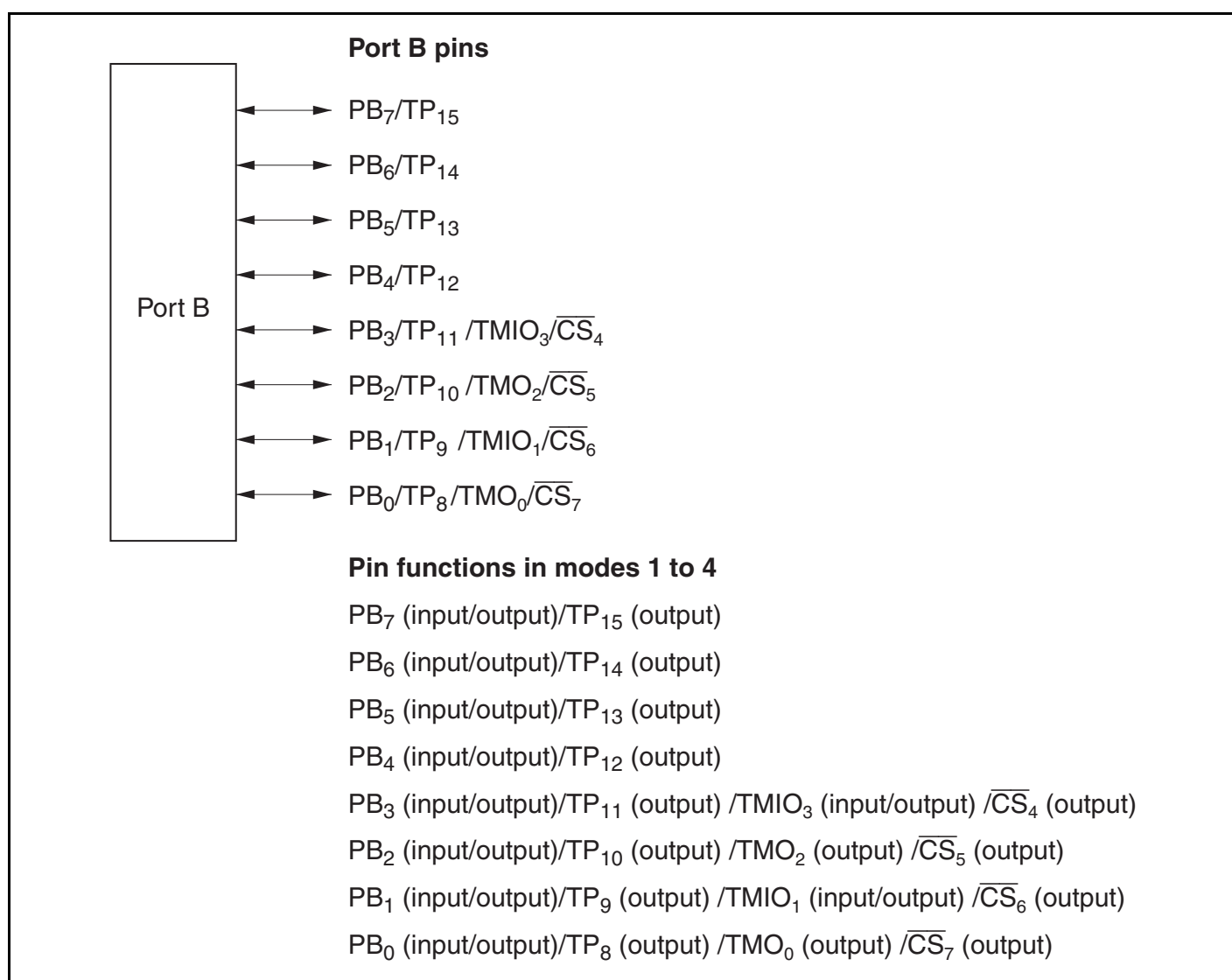
Figure 7.7 Port B Pin Configuration
