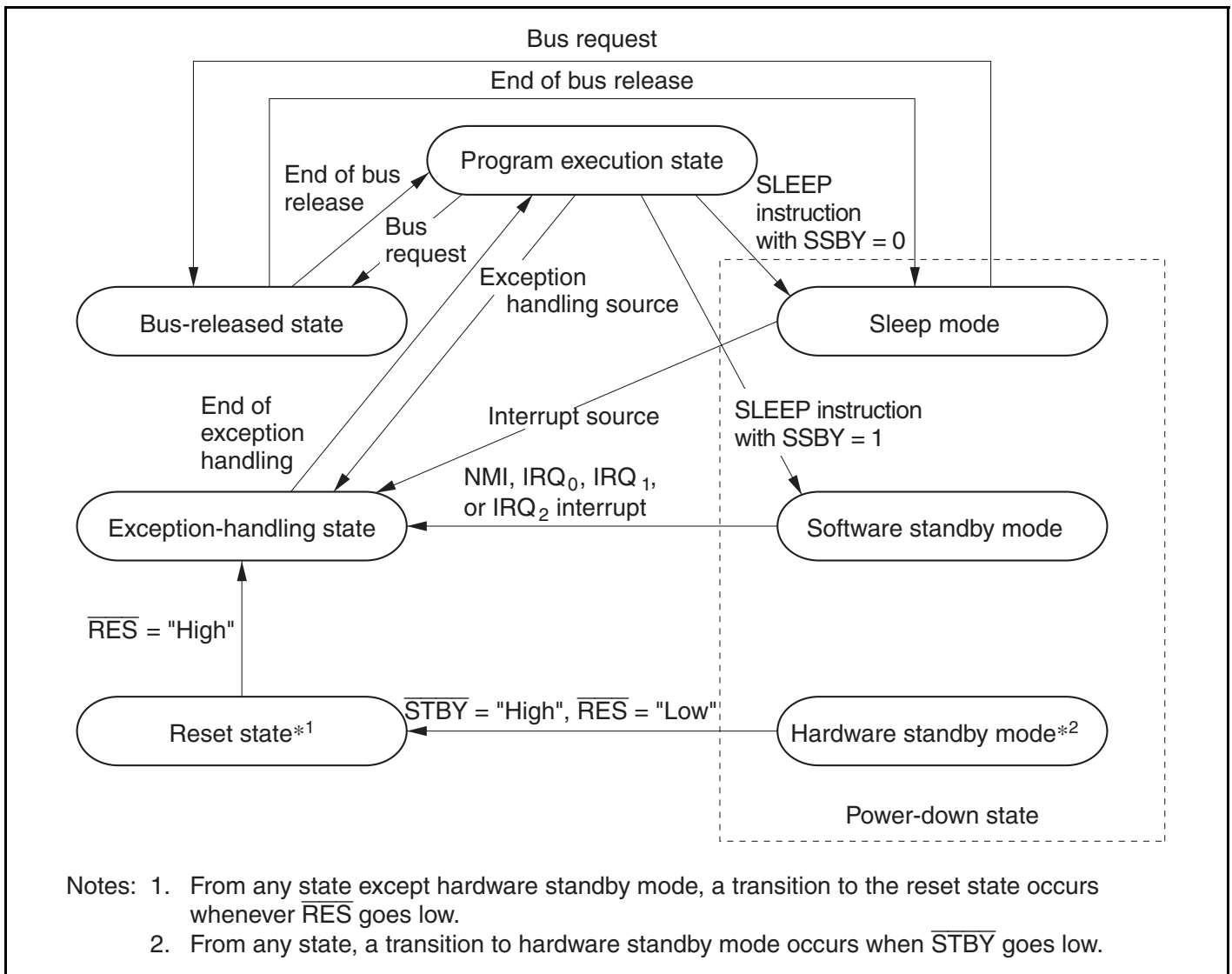
Figure 2.13 State Transitions
