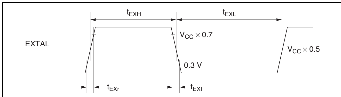
Figure 17.6 External Clock Input Timing
