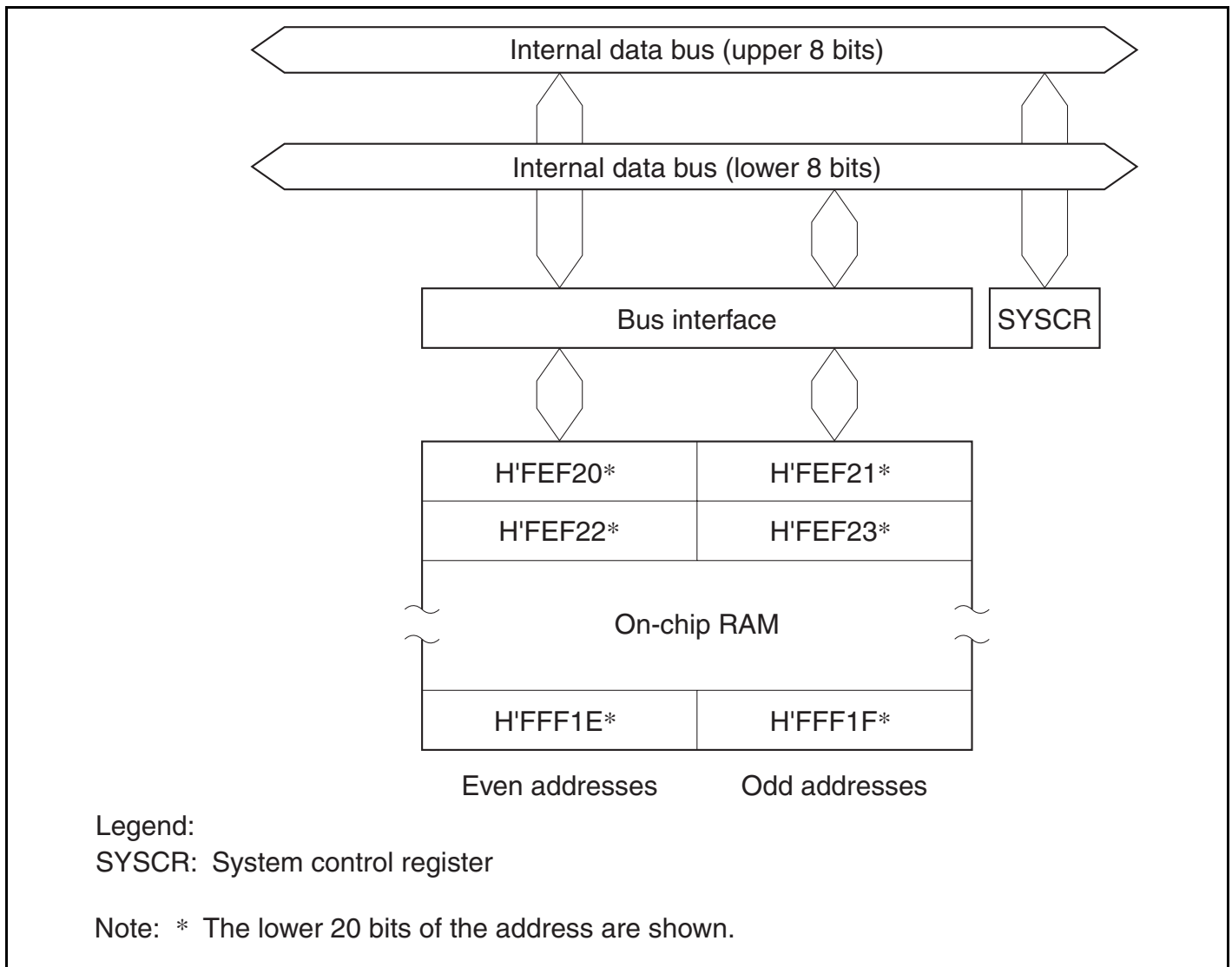
Figure 16.1 RAM Block Diagram
