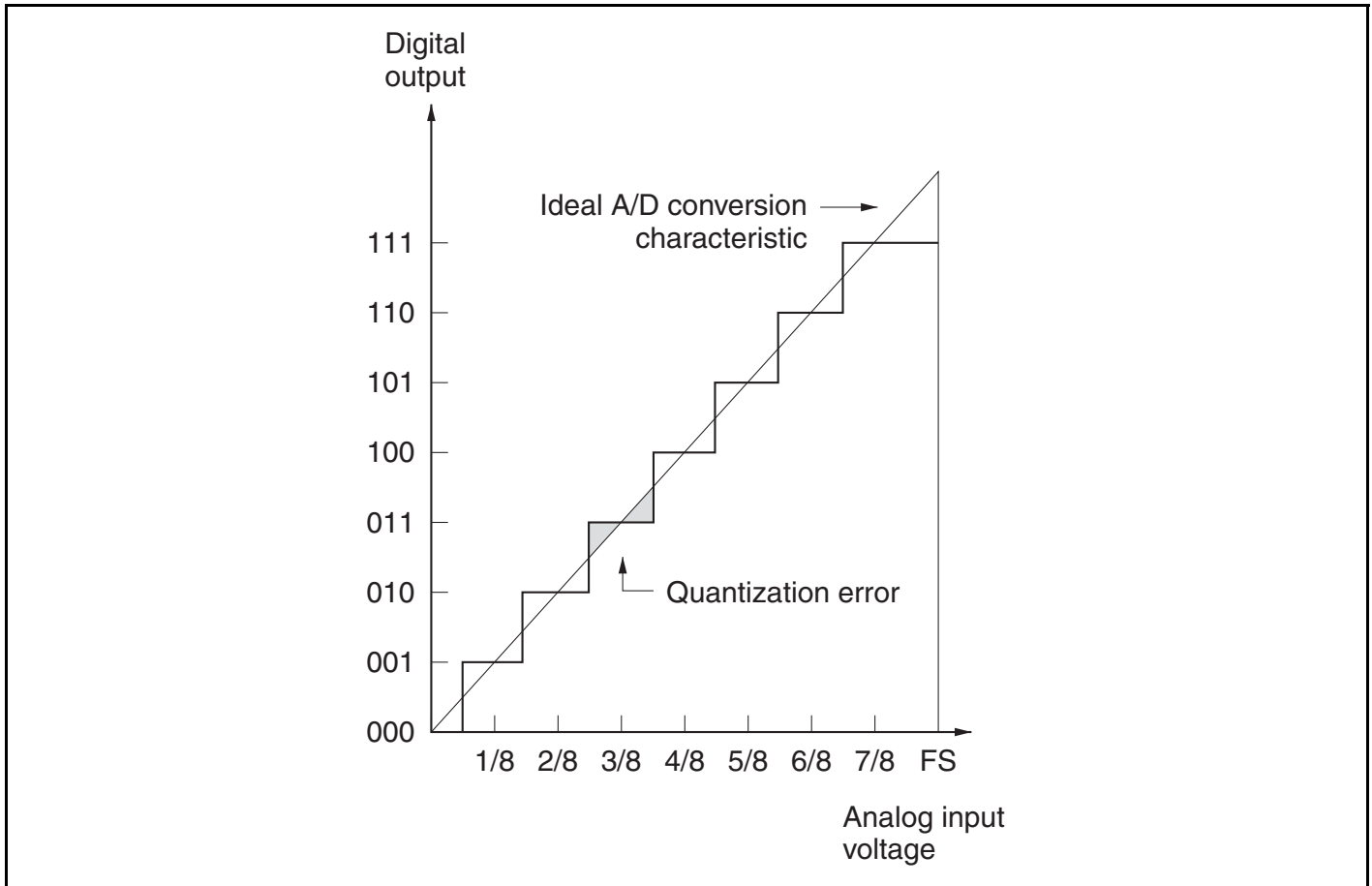
Figure 14.9 A/D Converter Accuracy Definitions (1)
