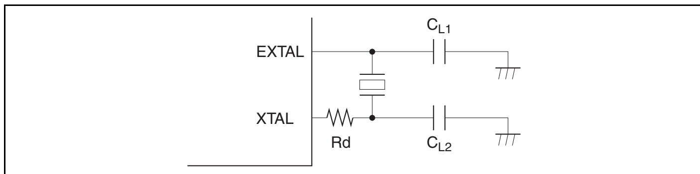
Figure 17.2 Connection of Crystal Resonator (Example)
