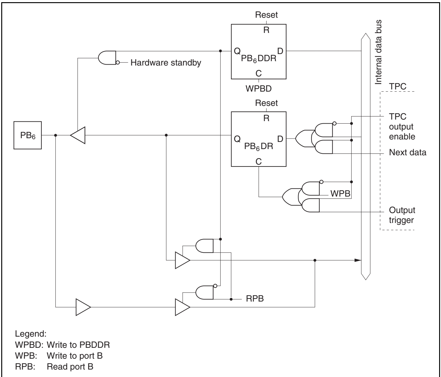
Figure C.7 (e) Port B Block Diagram (Pin PB 6 )
