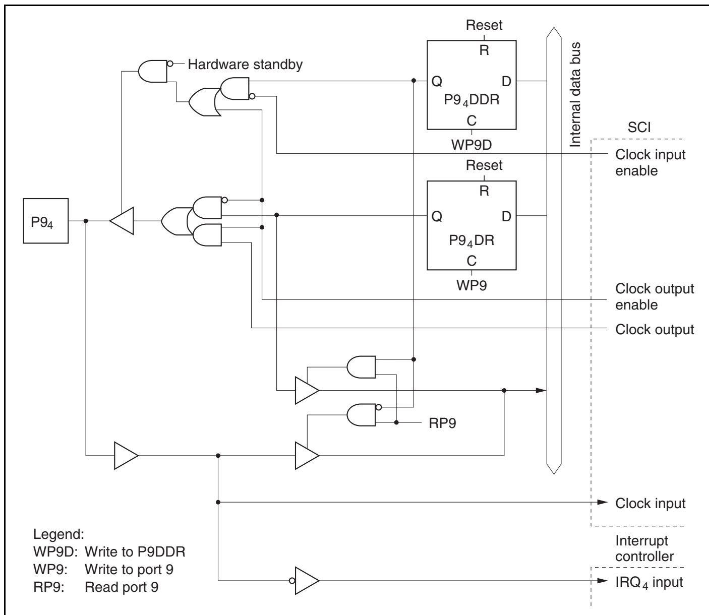
Figure C.5 (e) Port 9 Block Diagram (Pin P9 4 )
