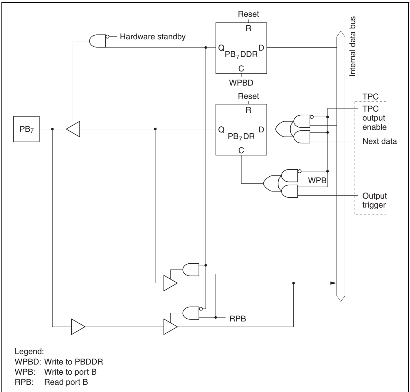
Figure C.7 (f) Port B Block Diagram (Pin PB 7 )
