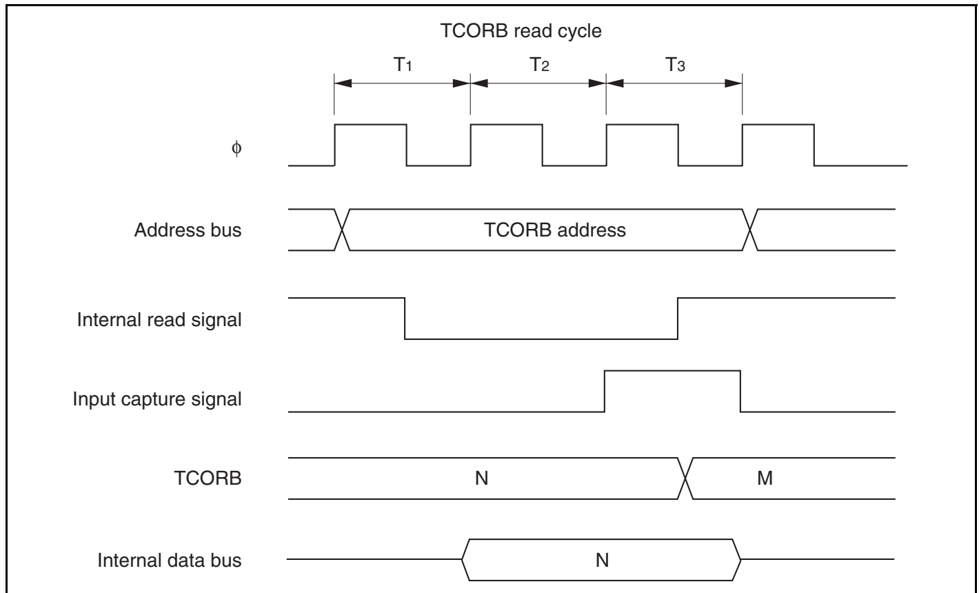
Figure 9.21 Contention between TCOR Read and Input Capture
