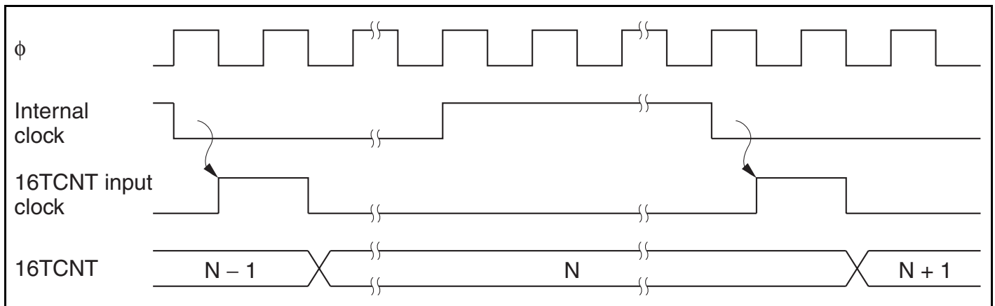
Figure 8.15 Count Timing for Internal Clock Sources
