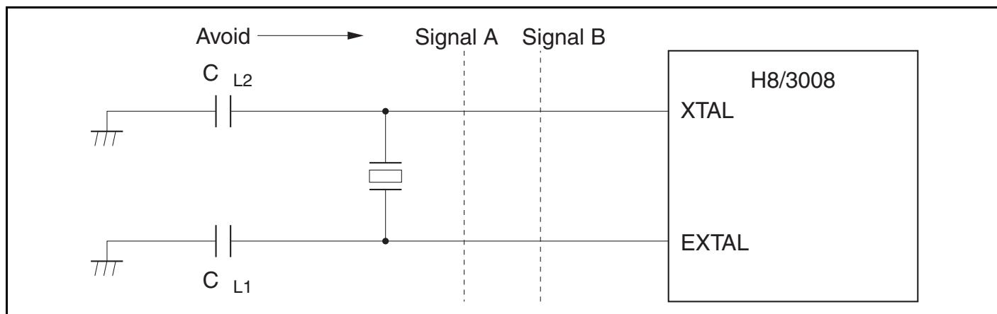
Figure 17.4 Oscillator Circuit Block Board Design Precautions
