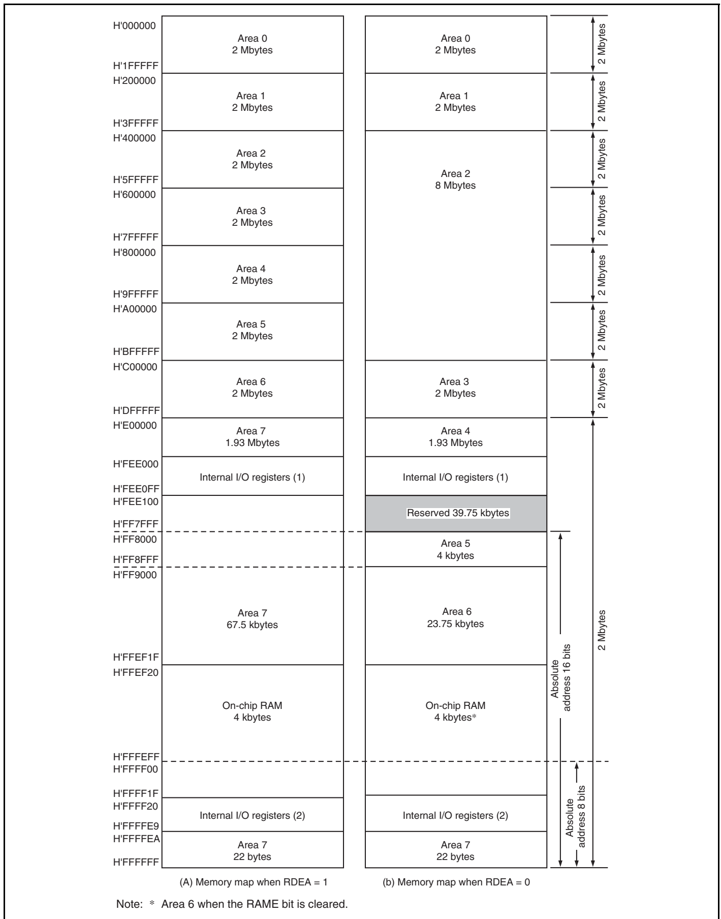
Figure 6.3 Memory Map in 16-Mbyte Mode
