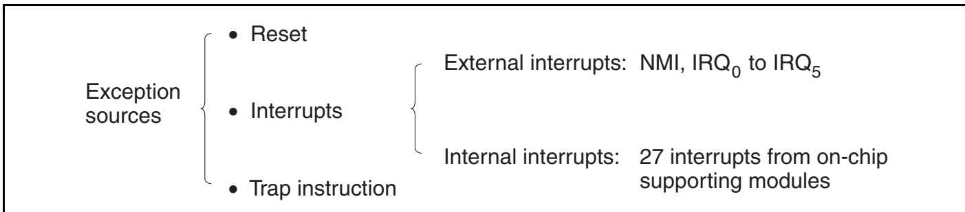
Figure 4.1 Exception Sources
