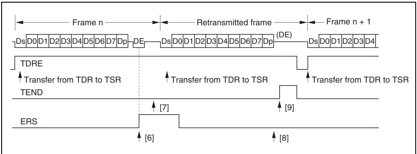
Figure 13.13 Retransmission in SCI Transmit Mode
