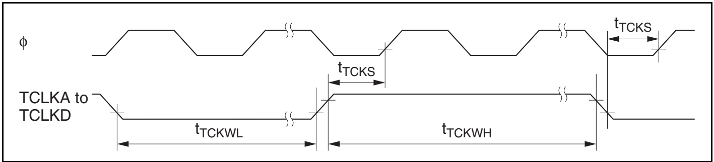
Figure 19.13 Timer External Clock Input Timing
