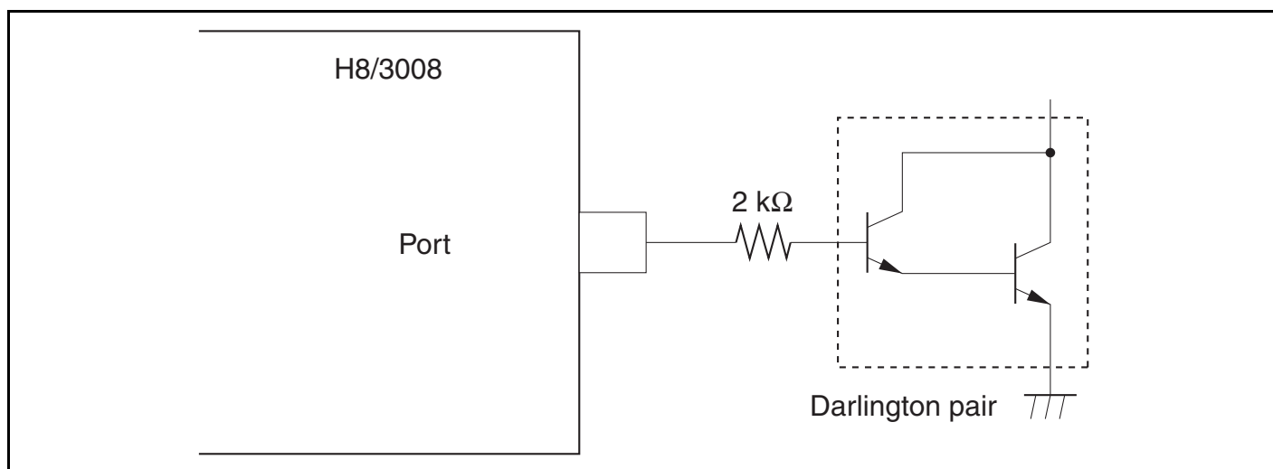
Figure 19.1 Darlington Pair Drive Circuit (Example)
