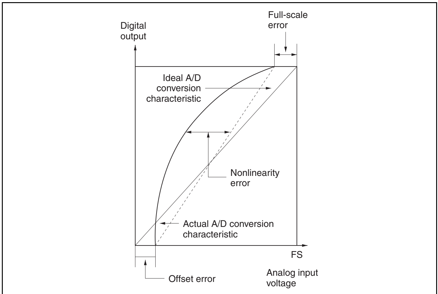
Figure 14.10 A/D Converter Accuracy Definitions (2)
