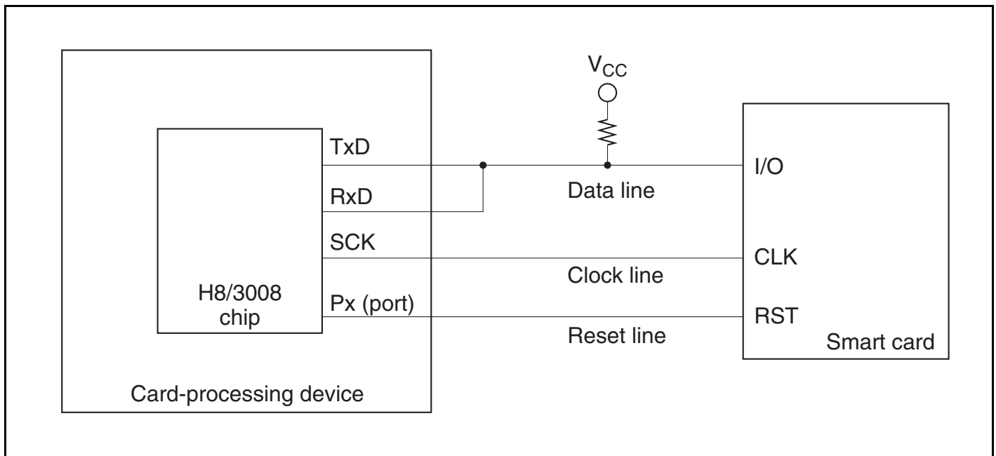
Figure 13.2 Smart Card Interface Connection Diagram
