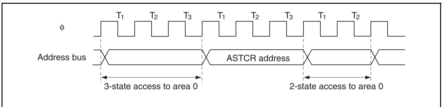
Figure 6.22 ASTCR Write Timing
