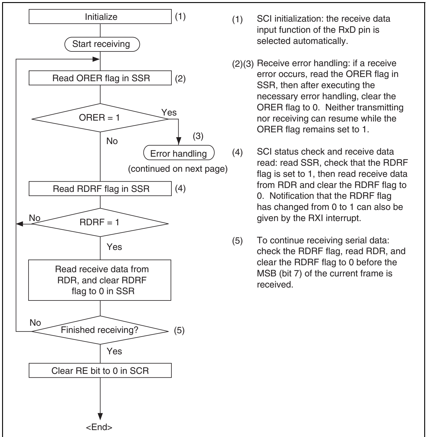
Figure 12.18 Sample Flowchart for Serial Receiving (1)
