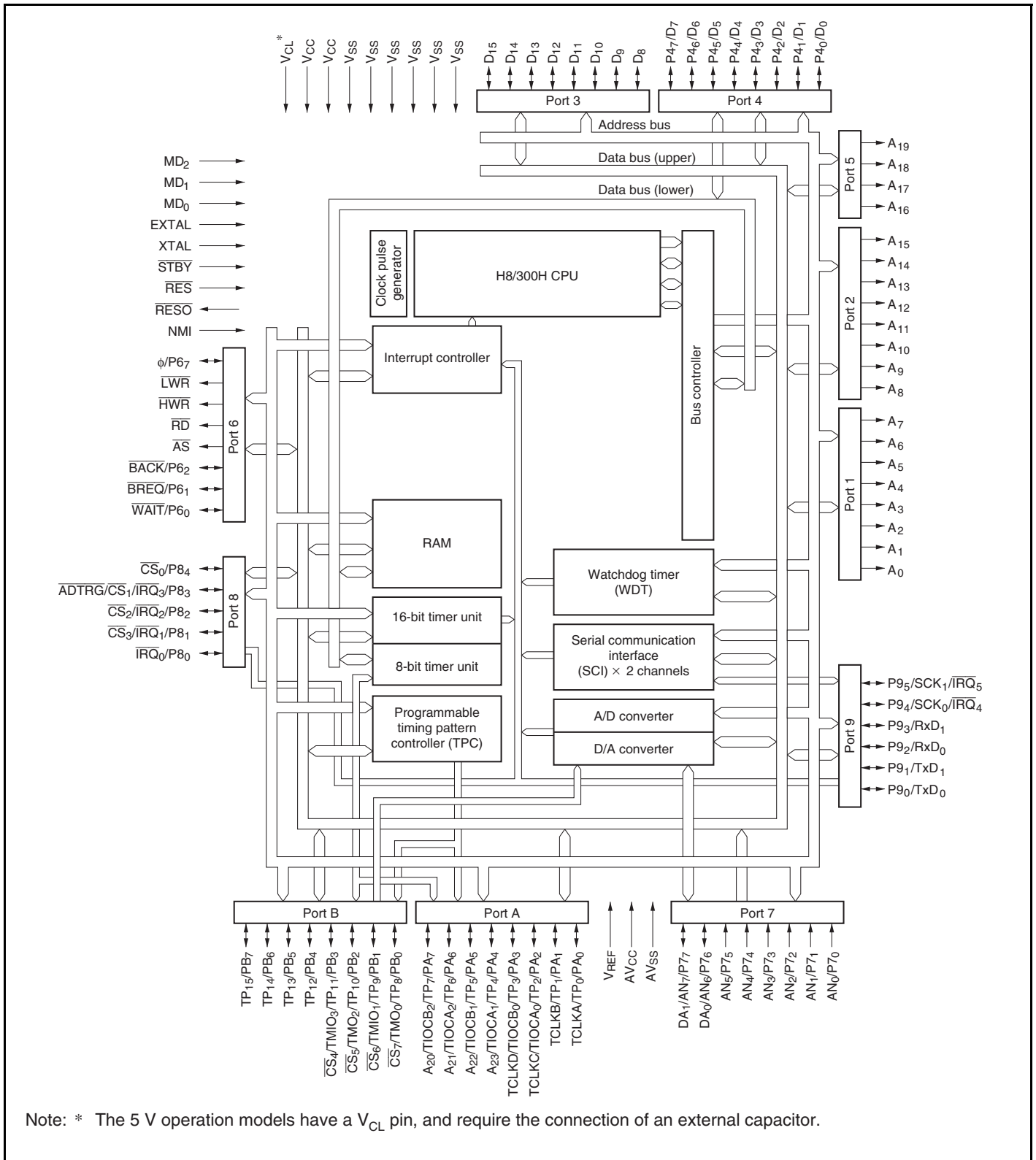
Figure 1.1 Block Diagram
