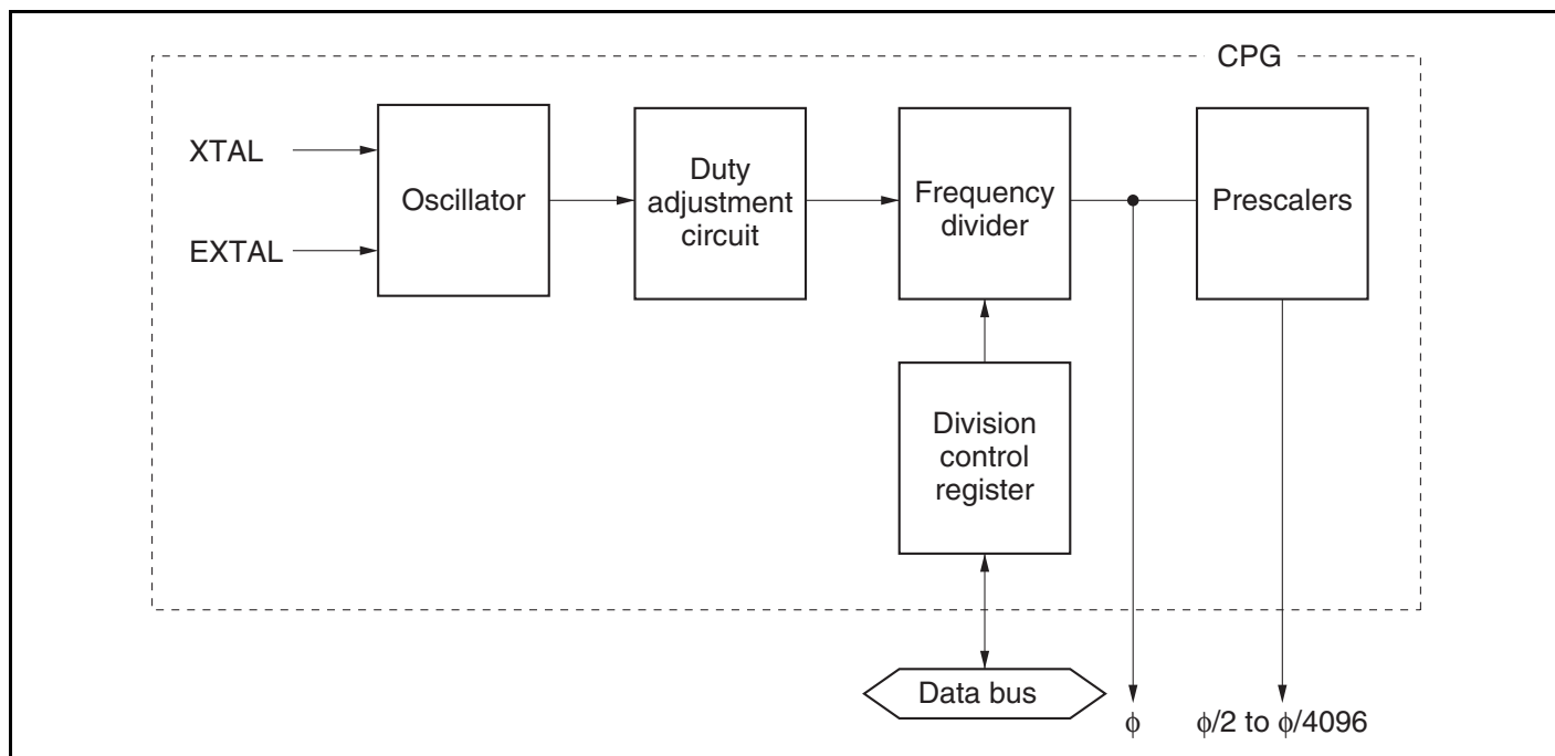
Figure 17.1 Block Diagram of Clock Pulse Generator
