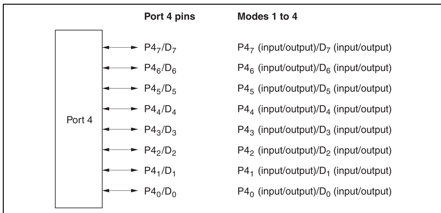
Figure 7.1 Port 4 Pin Configuration
