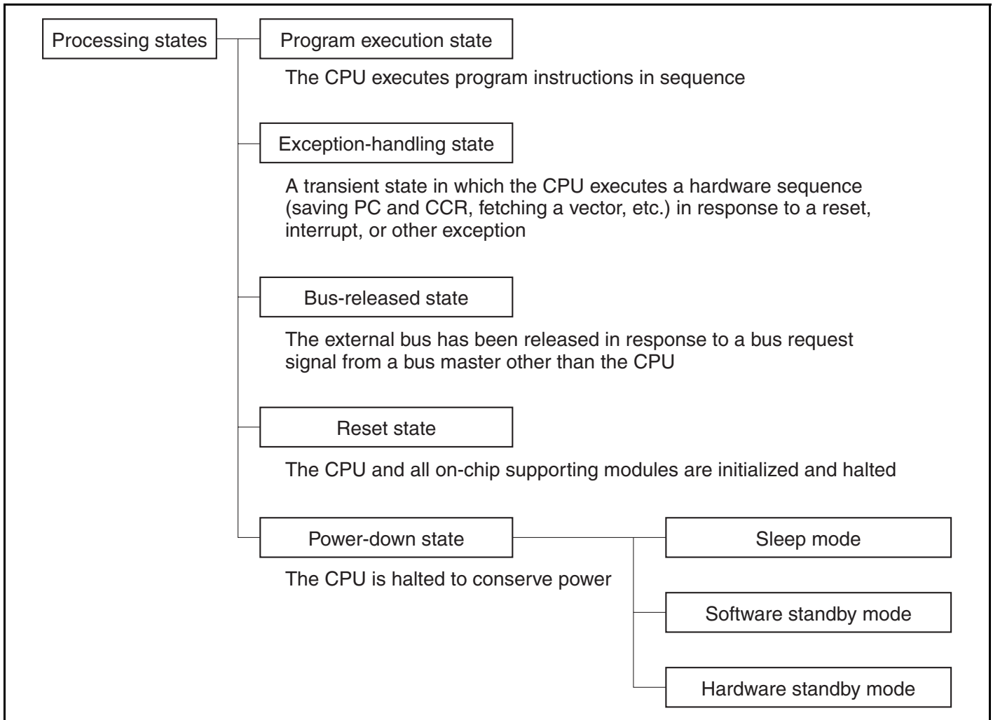
Figure 2.11 Processing States
