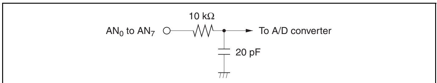
Figure 14.8 Analog Input Pin Equivalent Circuit
