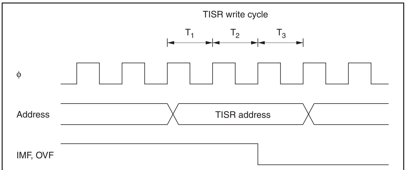
Figure 8.36 Timing of Clearing of Status Flags
