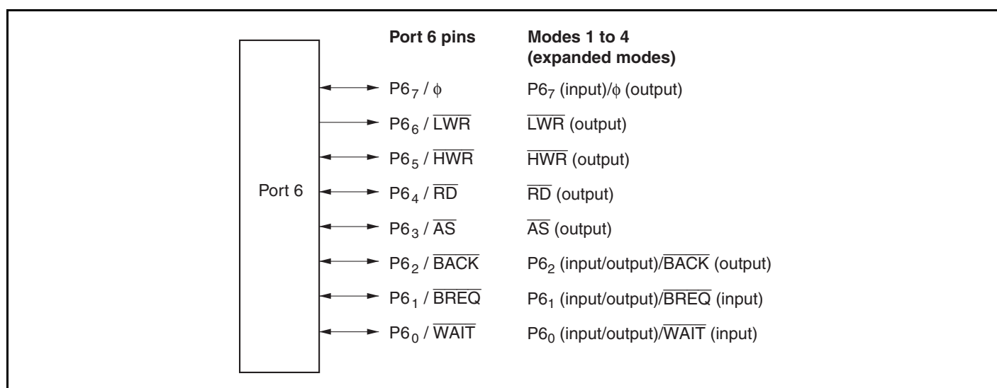
Figure 7.2 Port 6 Pin Configuration
