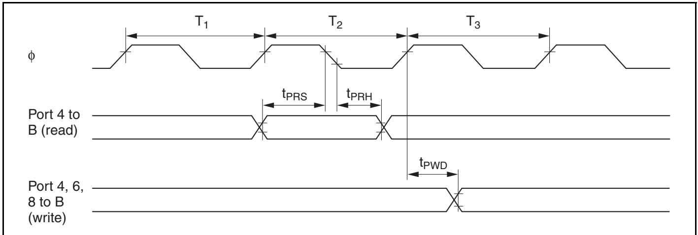
Figure 19.11 TPC and I/O Port Input/Output Timing
