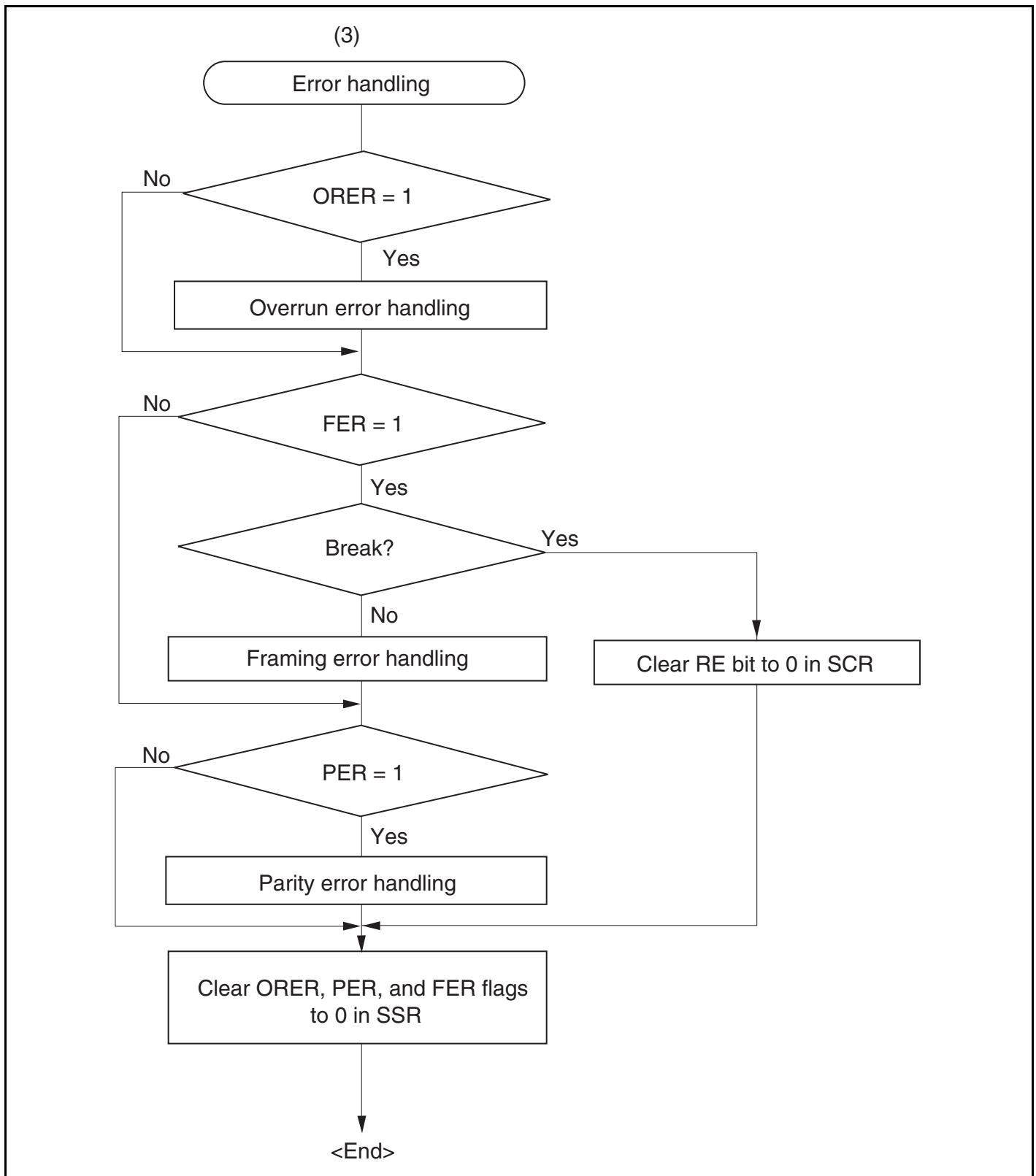
Figure 12.7 Sample Flowchart for Receiving Serial Data (2)
