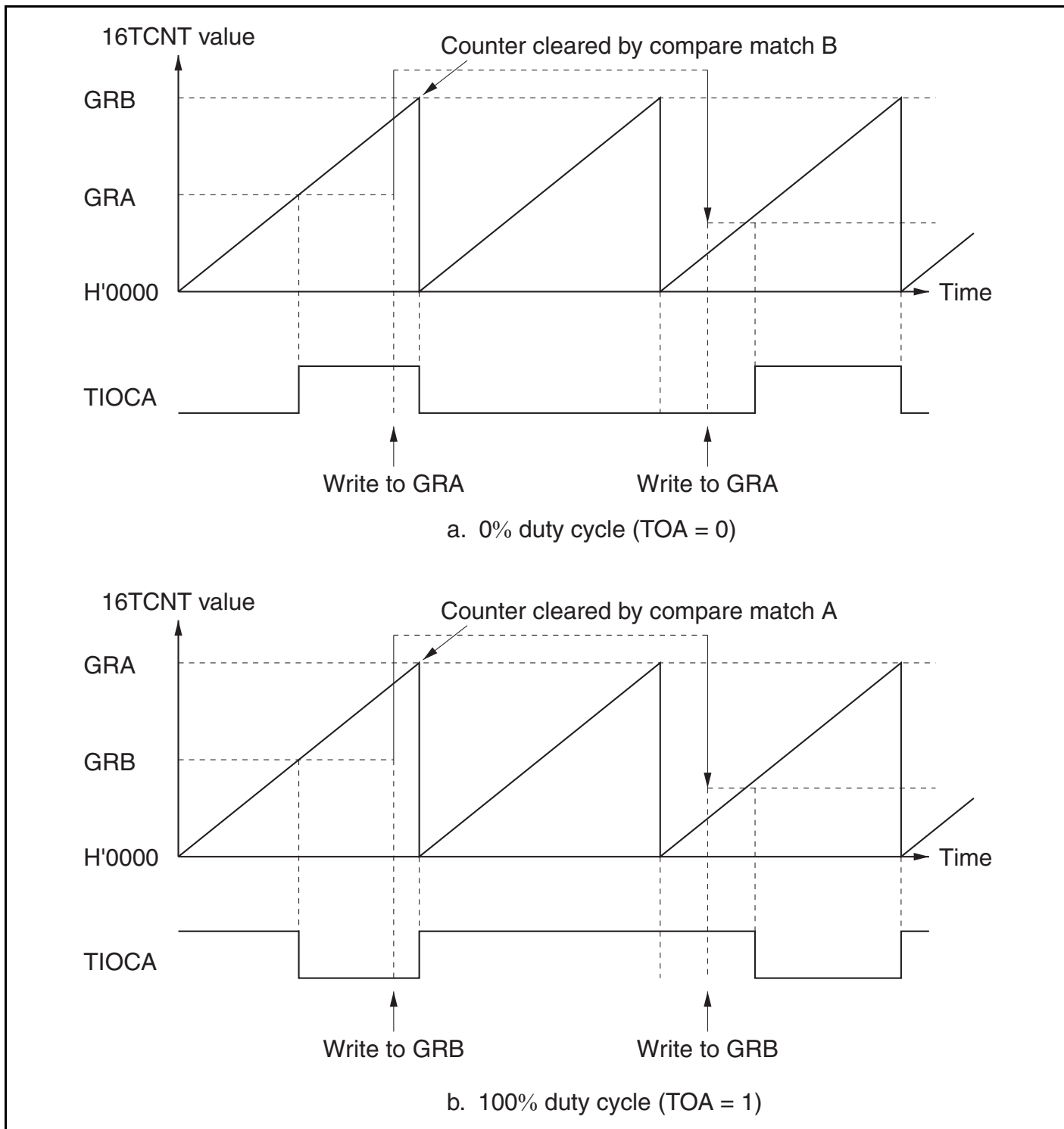
Figure 8.28 PWM Mode (Example 2)
