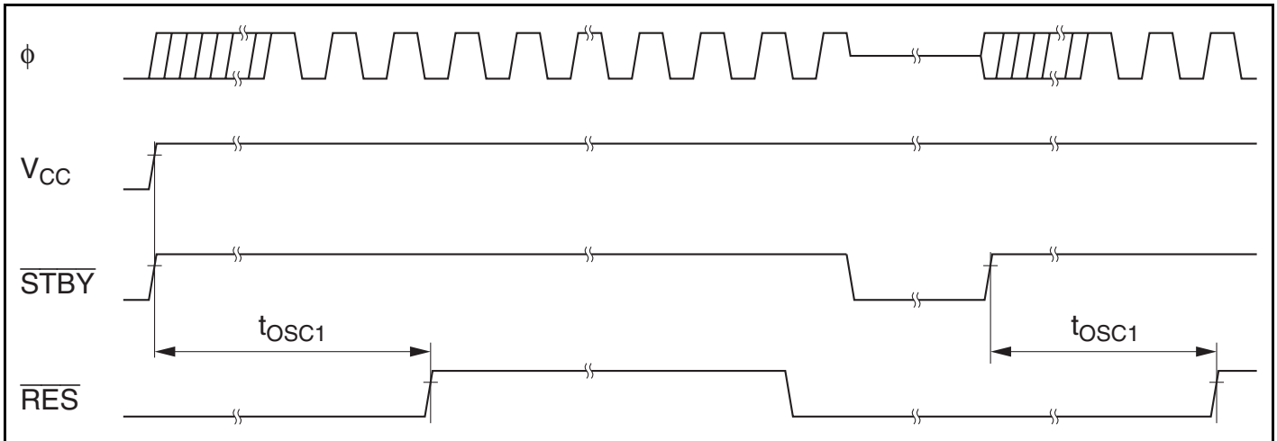
Figure 19.3 Oscillator Settling Timing
