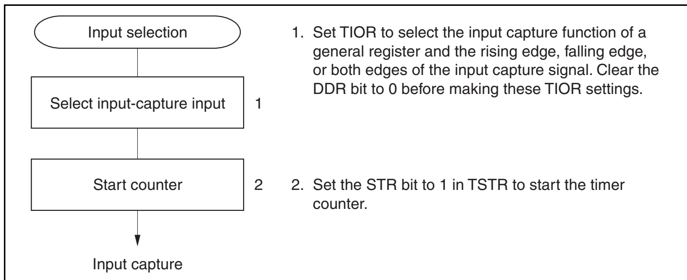
Figure 8.21 Setup Procedure for Input Capture (Example)
