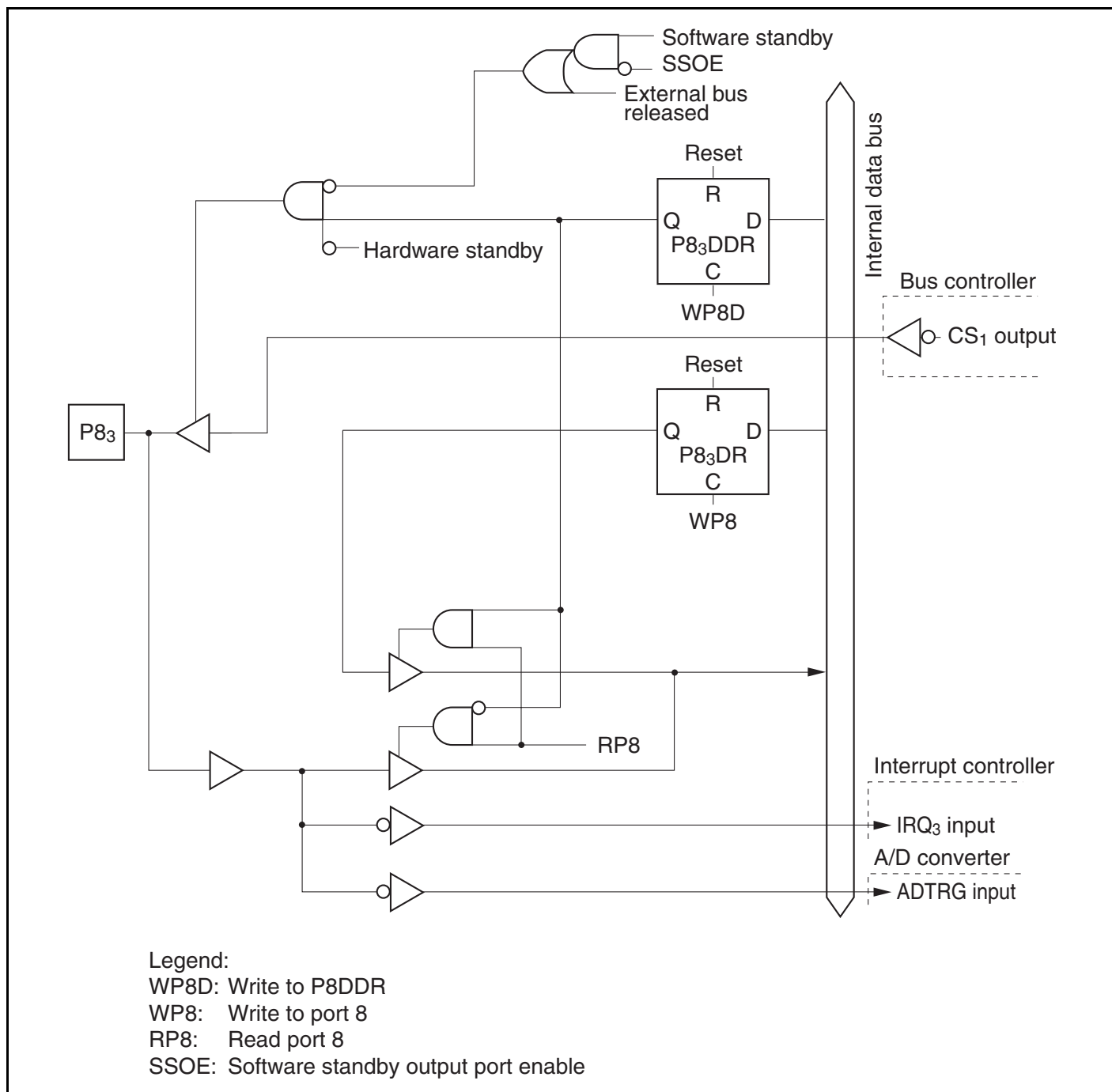
Figure C.4 (c) Port 8 Block Diagram (Pin P8 3 )
