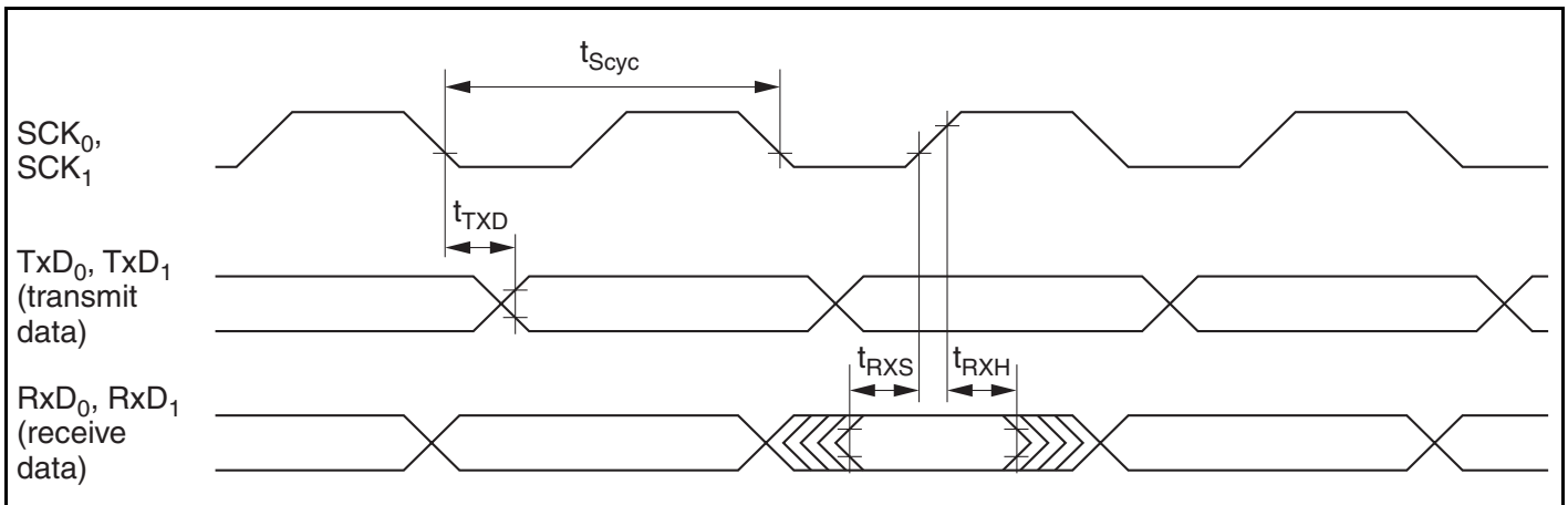
Figure 19.15 SCI Input/Output Timing in Synchronous Mode
