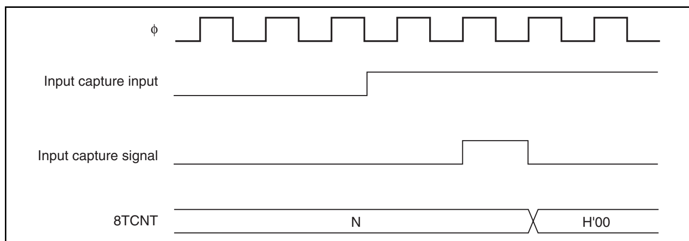
Figure 9.12 Timing of Clear by Input Capture
