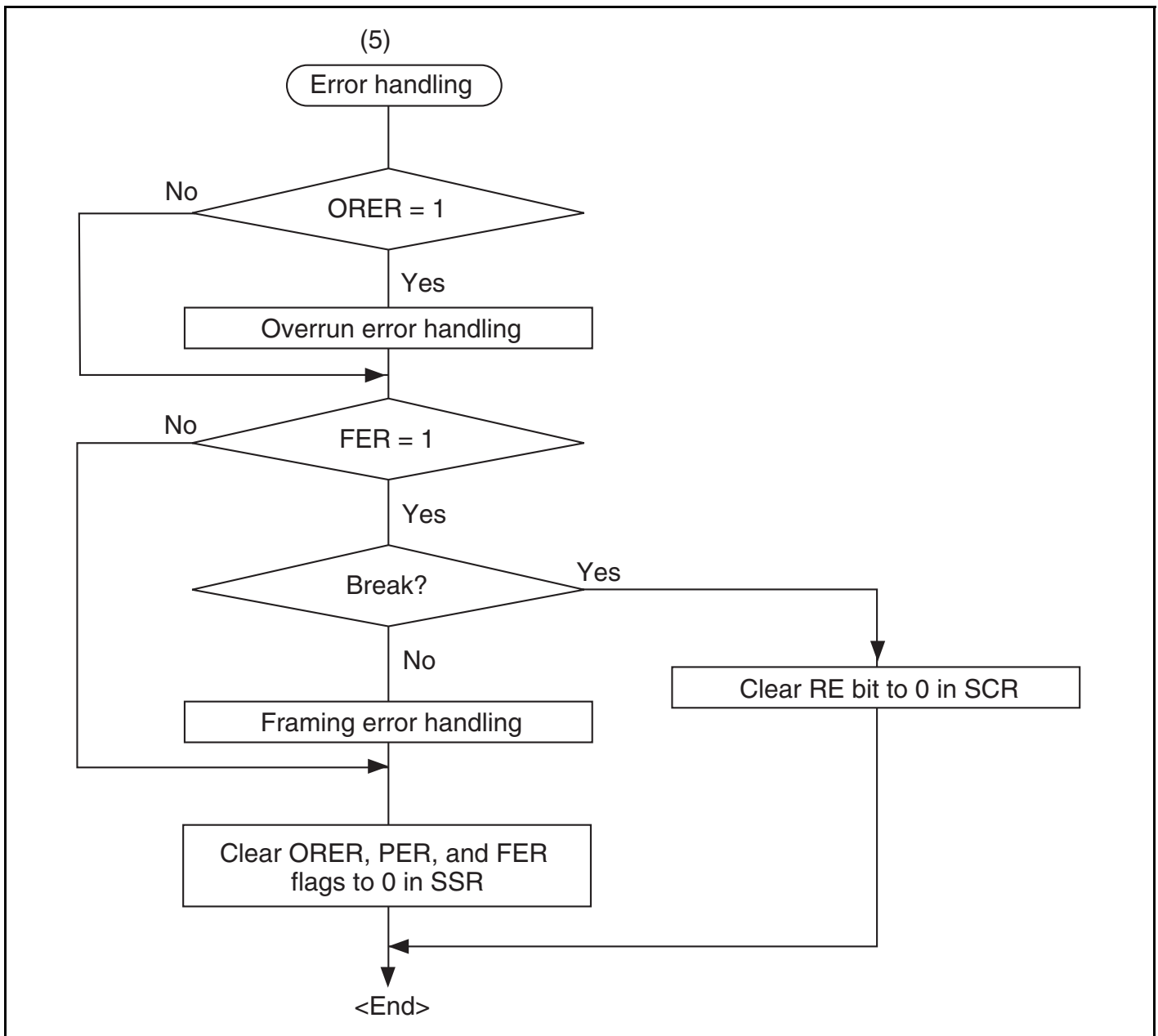
Figure 12.12 Sample Flowchart for Receiving Multiprocessor Serial Data (2)
