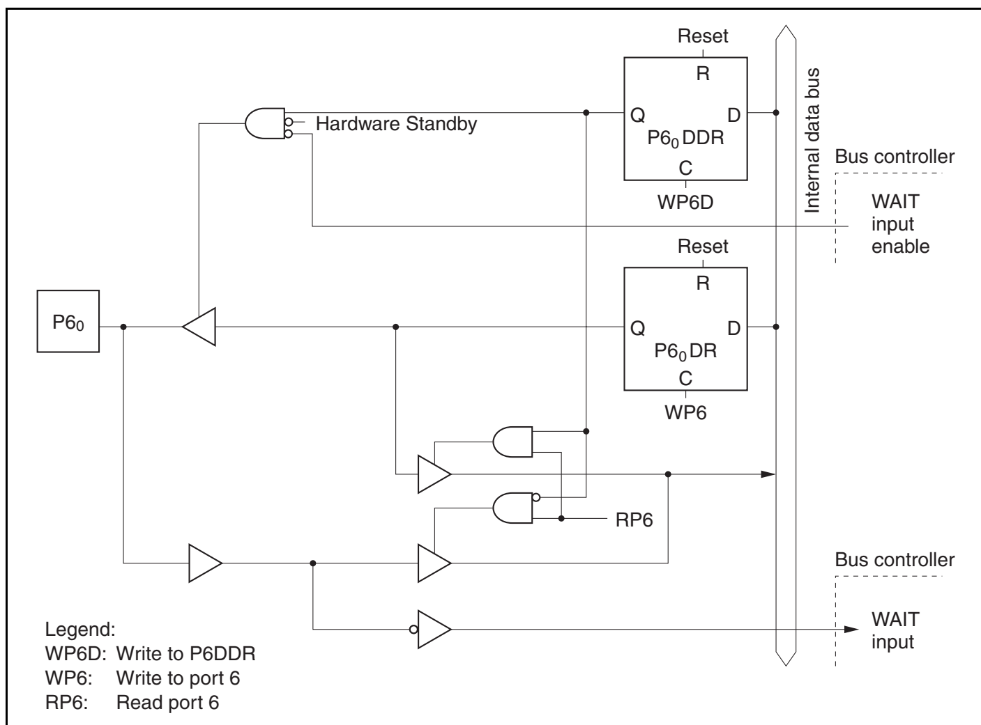
Figure C.2 (a) Port 6 Block Diagram (Pin P6 0 )
