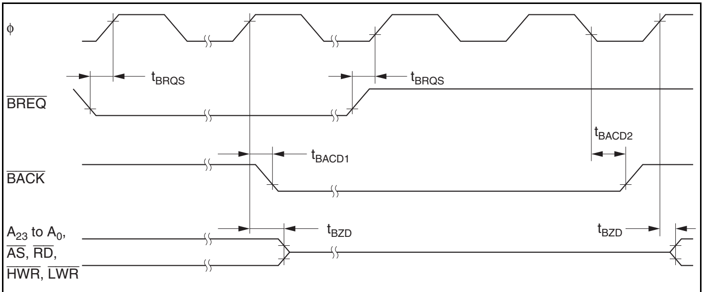
Figure 19.10 Bus-Release Mode Timing
