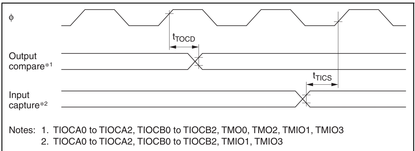
Figure 19.12 Timer Input/Output Timing
