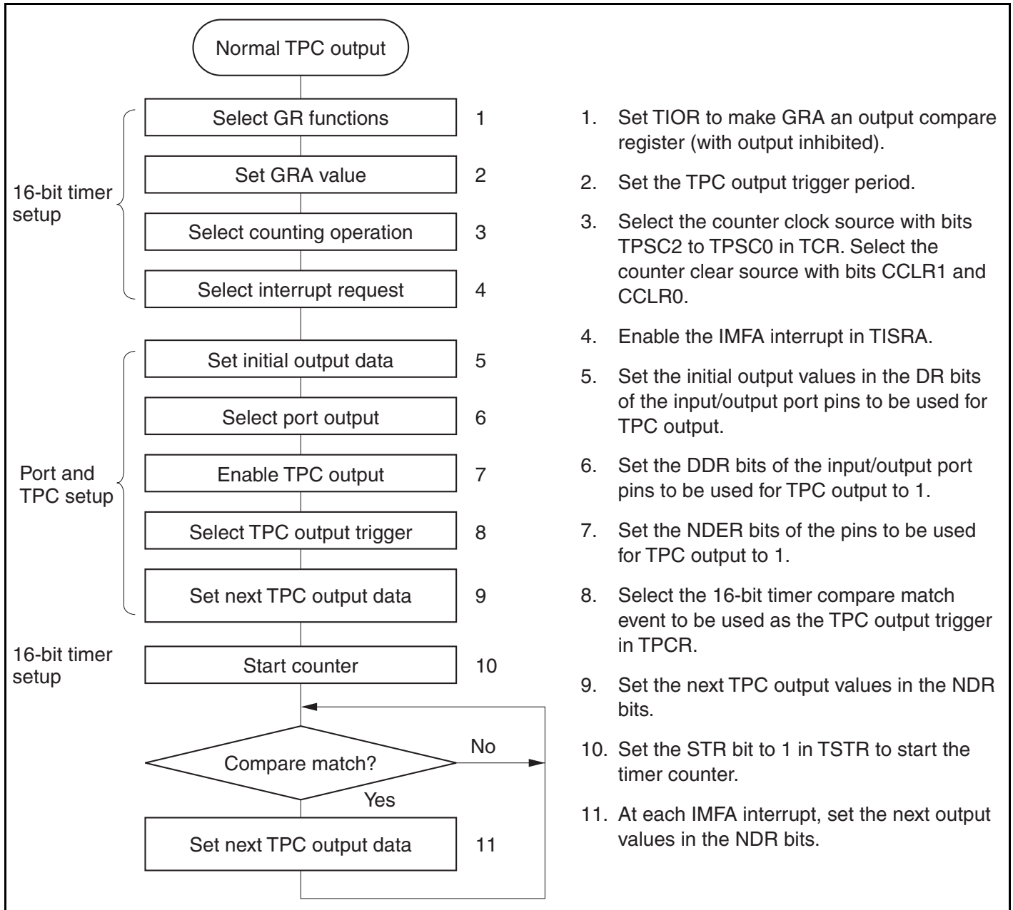
Figure 10.4 Setup Procedure for Normal TPC Output (Example)
