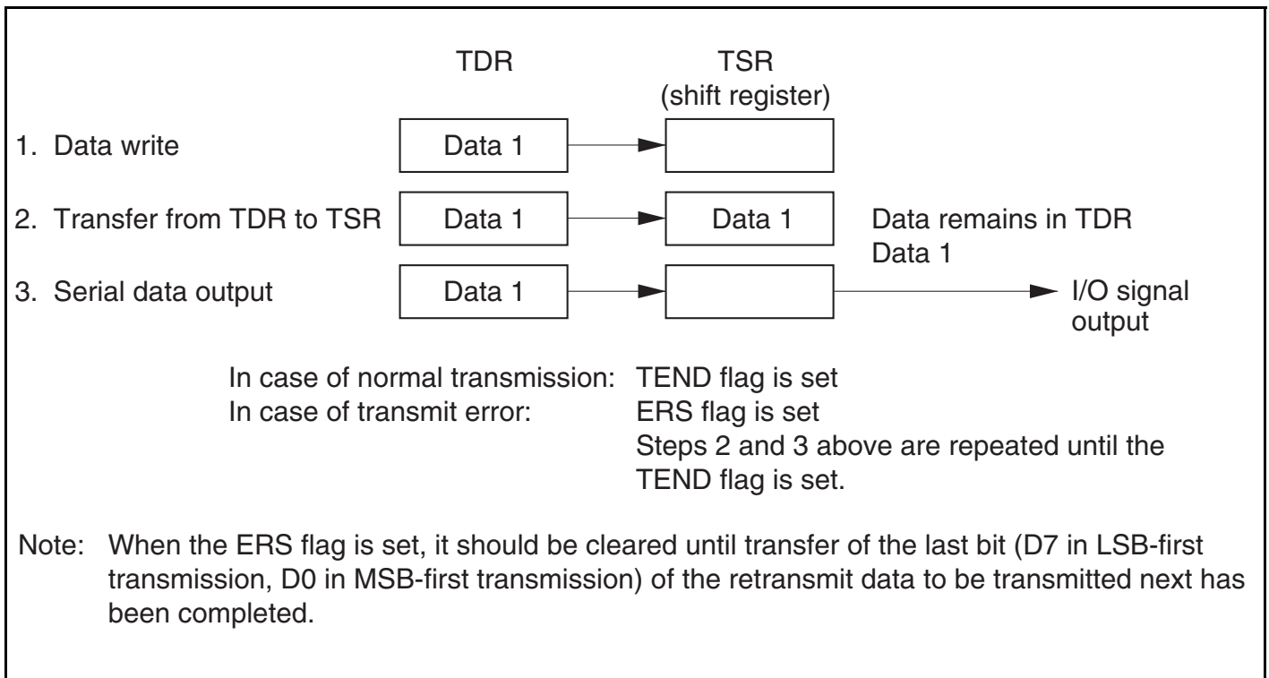
Figure 13.6 Relation Between Transmit Operation and Internal Registers
