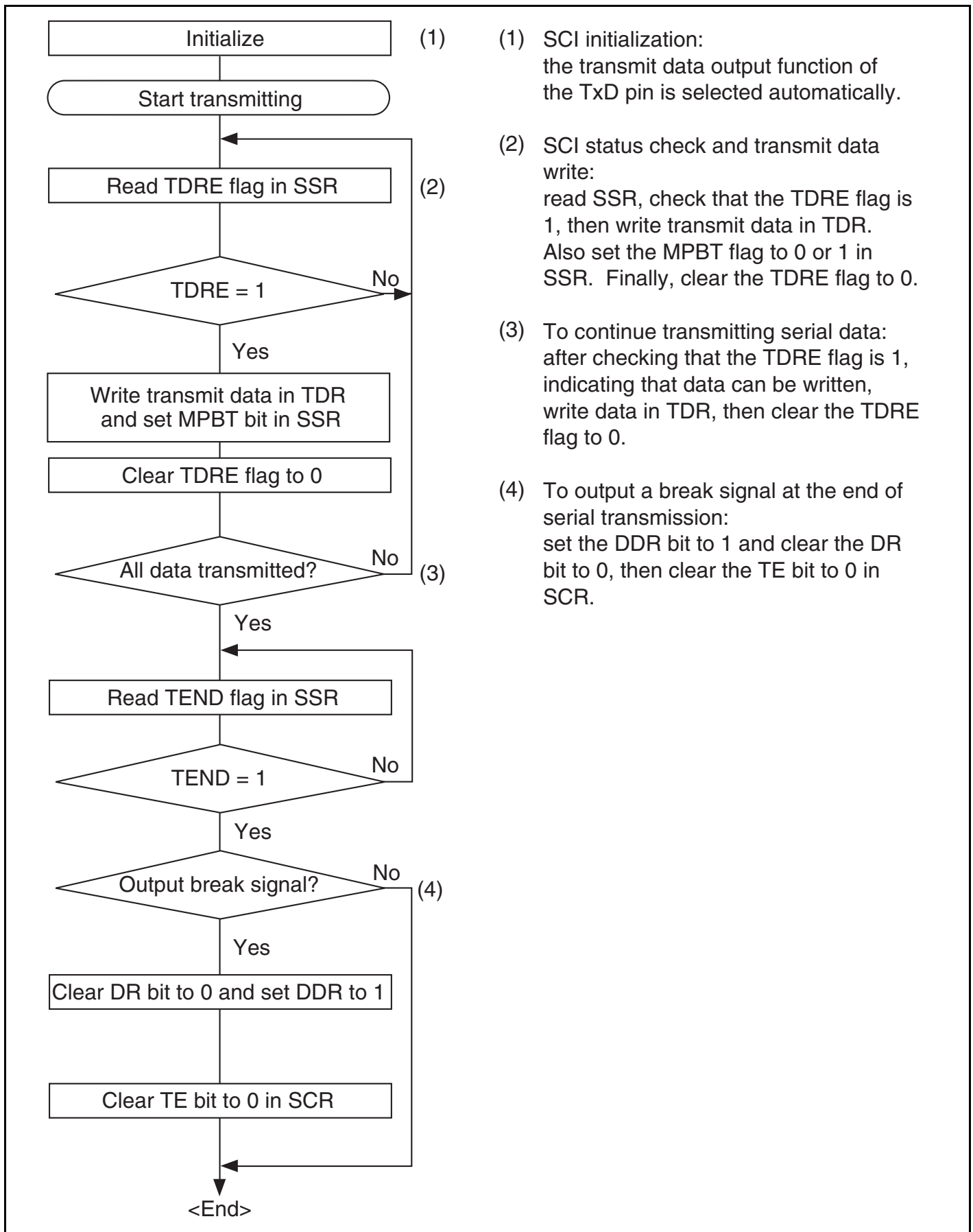
Figure 12.10 Sample Flowchart for Transmitting Multiprocessor Serial Data
